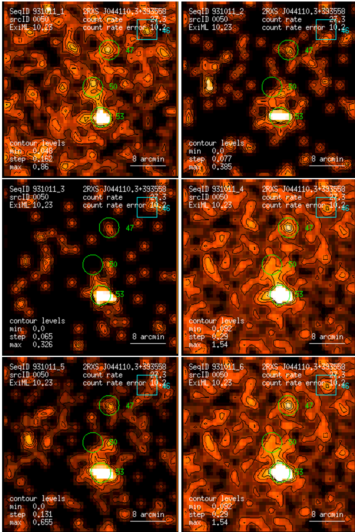
Figure 50: RASS 931011: detection 0050: band rate images, Gaussian filter: (1) PSPC channels 11 – 41, (2) 52 – 90, (3) 91 – 201, (4) 11 – 235, (5) 52 – 201, (6) 11 – 201. Broad band rates in counts/ks. Band rate contour levels in counts/ks/arcmin 2 .
