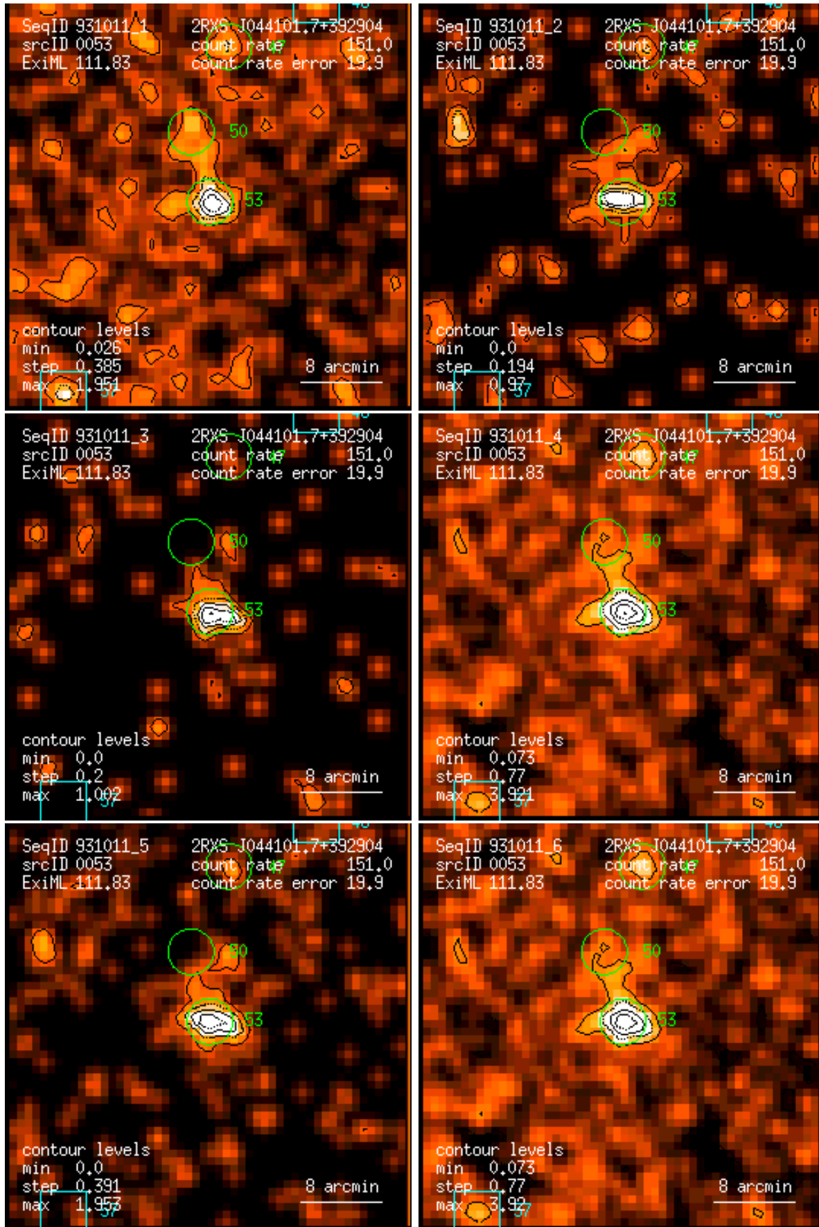
Figure 53: RASS 931011: detection 0053: band rate images, Gaussian filter: (1) PSPC channels 11 – 41, (2) 52 – 90, (3) 91 – 201, (4) 11 – 235, (5) 52 – 201, (6) 11 – 201. Broad band rates in counts/ks. Band rate contour levels in counts/ks/arcmin 2 .
