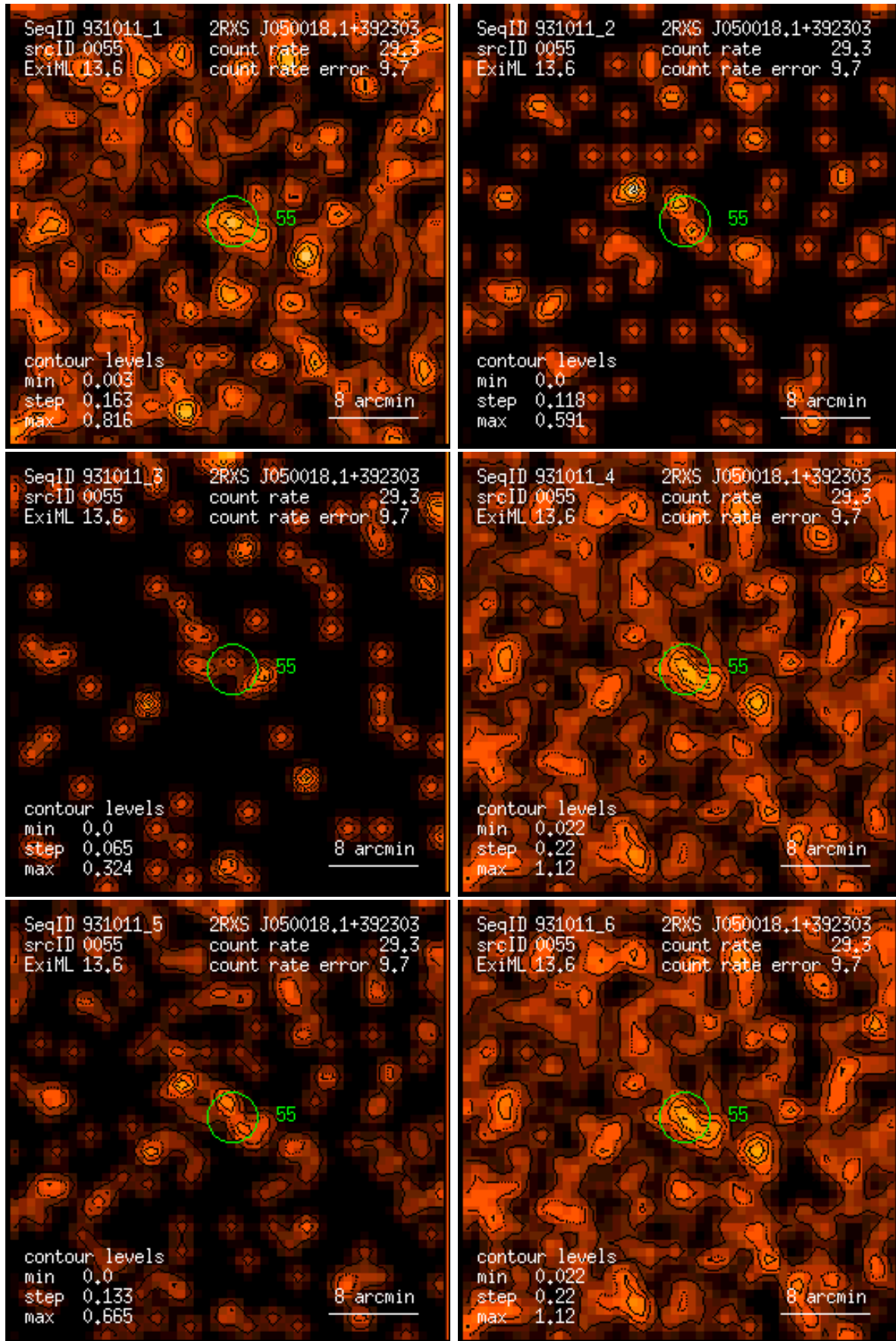
Figure 55: RASS 931011: detection 0055: band rate images, Gaussian filter: (1) PSPC channels 11 – 41, (2) 52 – 90, (3) 91 – 201, (4) 11 – 235, (5) 52 – 201, (6) 11 – 201. Broad band rates in counts/ks. Band rate contour levels in counts/ks/arcmin 2 .
