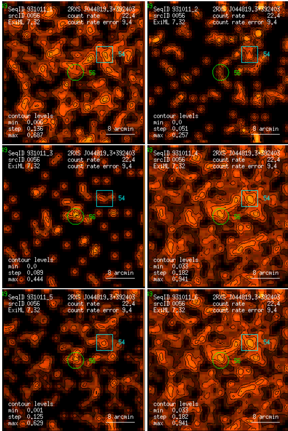
Figure 56: RASS 931011: detection 0056: band rate images, Gaussian filter: (1) PSPC channels 11 – 41, (2) 52 – 90, (3) 91 – 201, (4) 11 – 235, (5) 52 – 201, (6) 11 – 201. Broad band rates in counts/ks. Band rate contour levels in counts/ks/arcmin 2 .
