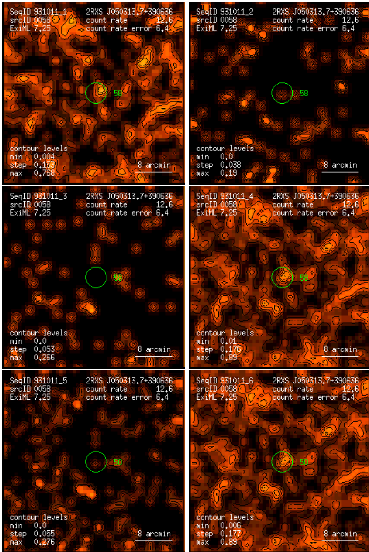
Figure 58: RASS 931011: detection 0058: band rate images, Gaussian filter: (1) PSPC channels 11 – 41, (2) 52 – 90, (3) 91 – 201, (4) 11 – 235, (5) 52 – 201, (6) 11 – 201. Broad band rates in counts/ks. Band rate contour levels in counts/ks/arcmin 2 .
