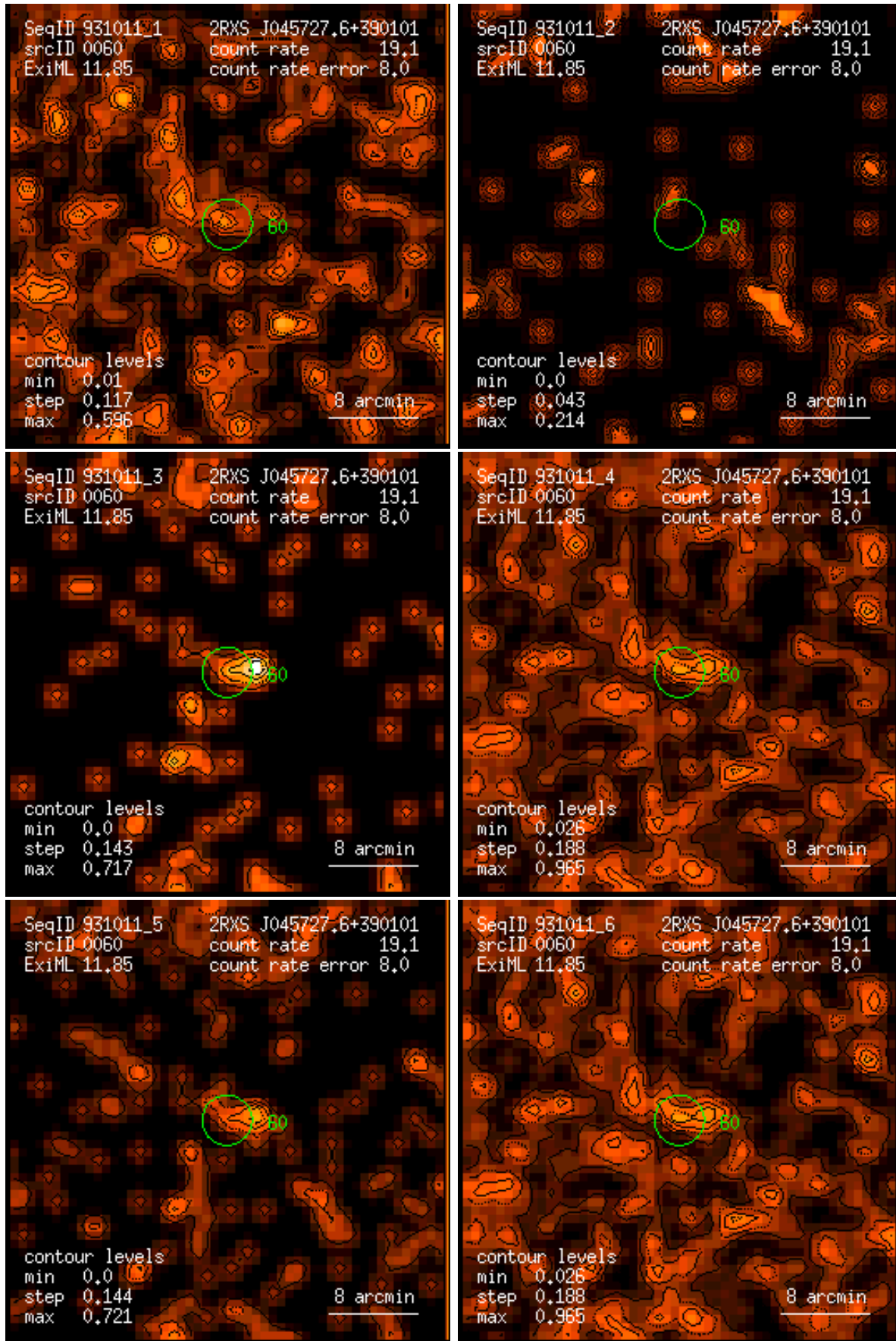
Figure 60: RASS 931011: detection 0060: band rate images, Gaussian filter: (1) PSPC channels 11 – 41, (2) 52 – 90, (3) 91 – 201, (4) 11 – 235, (5) 52 – 201, (6) 11 – 201. Broad band rates in counts/ks. Band rate contour levels in counts/ks/arcmin 2 .
