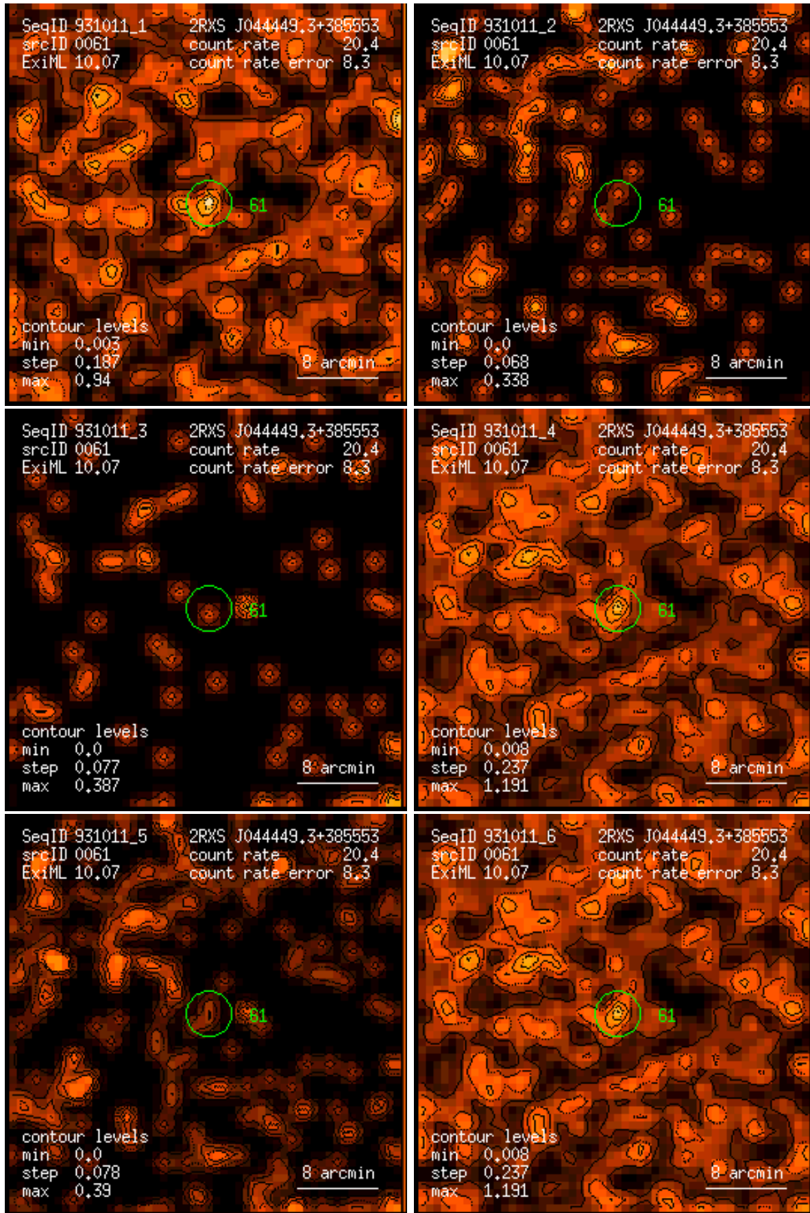
Figure 61: RASS 931011: detection 0061: band rate images, Gaussian filter: (1) PSPC channels 11 – 41, (2) 52 – 90, (3) 91 – 201, (4) 11 – 235, (5) 52 – 201, (6) 11 – 201. Broad band rates in counts/ks. Band rate contour levels in counts/ks/arcmin 2 .
