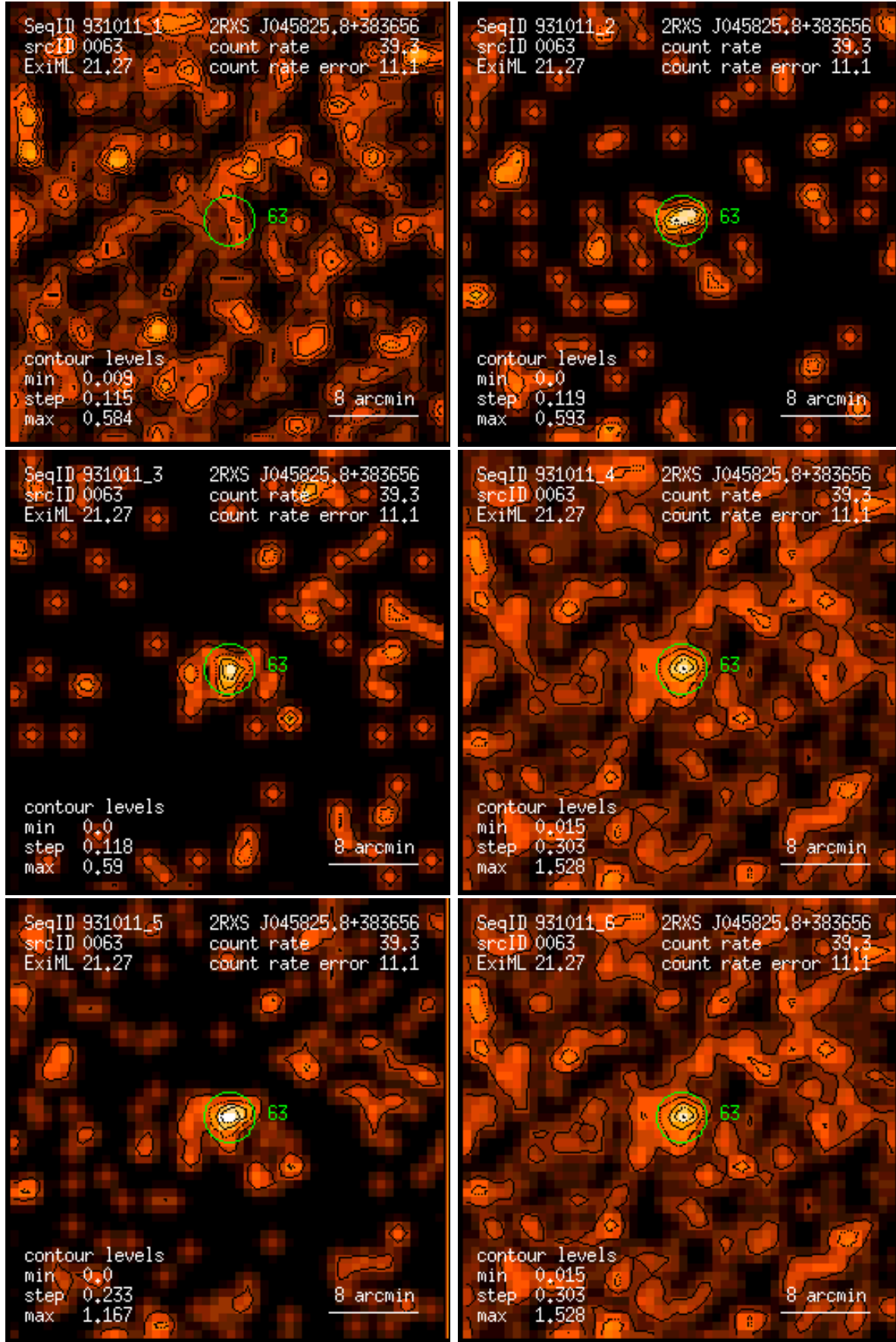
Figure 63: RASS 931011: detection 0063: band rate images, Gaussian filter: (1) PSPC channels 11 – 41, (2) 52 – 90, (3) 91 – 201, (4) 11 – 235, (5) 52 – 201, (6) 11 – 201. Broad band rates in counts/ks. Band rate contour levels in counts/ks/arcmin 2 .
