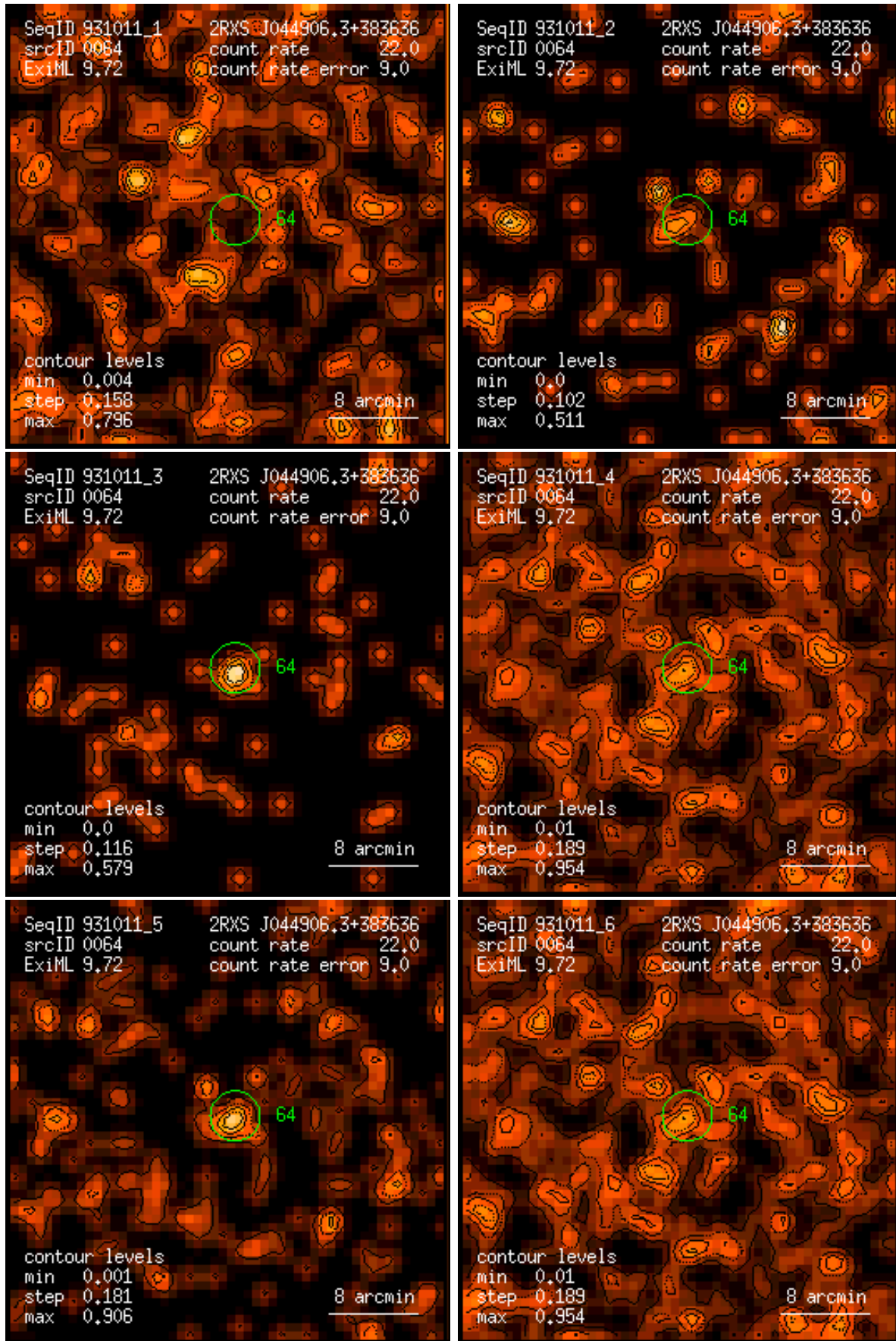
Figure 64: RASS 931011: detection 0064: band rate images, Gaussian filter: (1) PSPC channels 11 – 41, (2) 52 – 90, (3) 91 – 201, (4) 11 – 235, (5) 52 – 201, (6) 11 – 201. Broad band rates in counts/ks. Band rate contour levels in counts/ks/arcmin 2 .
