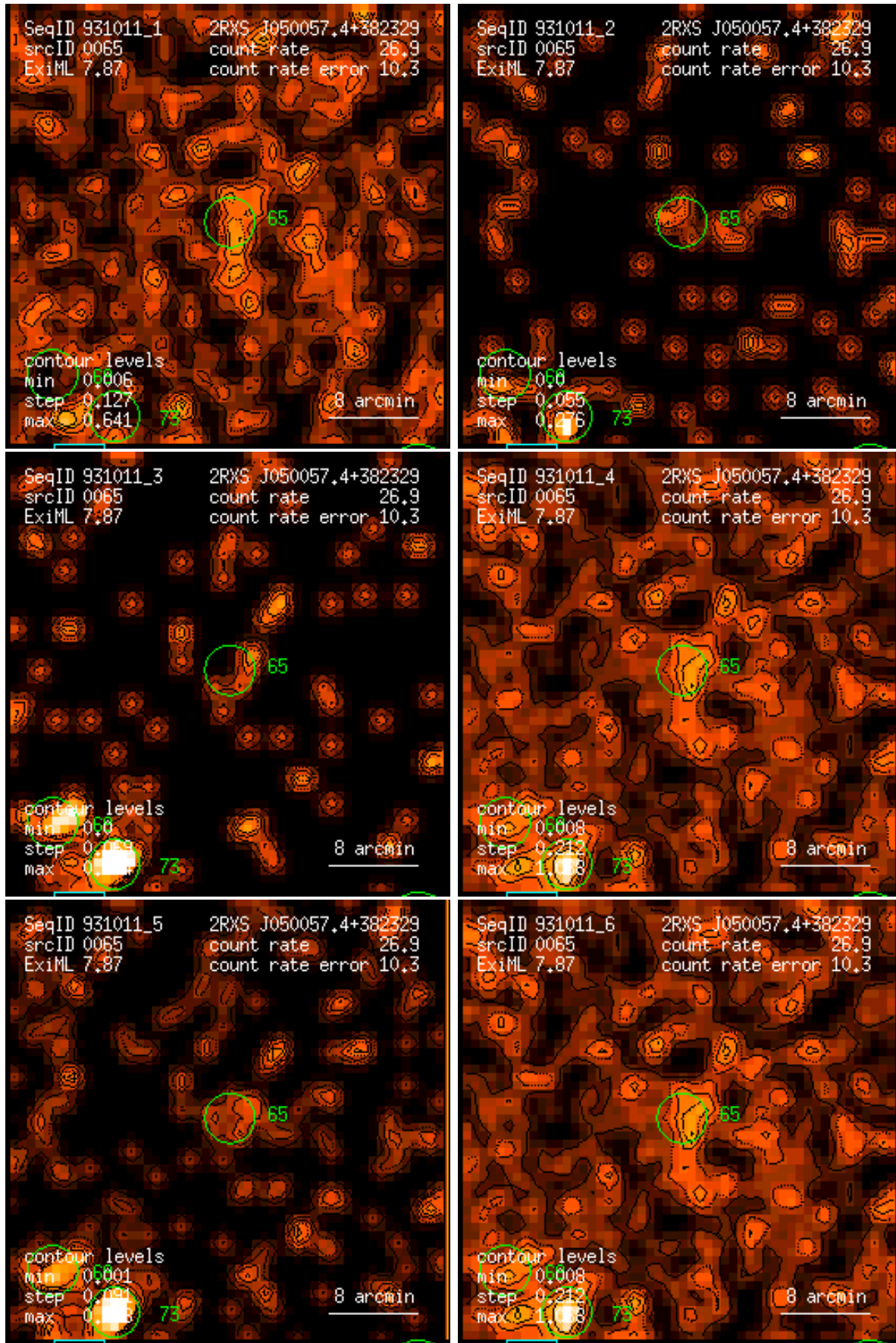
Figure 65: RASS 931011: detection 0065: band rate images, Gaussian filter: (1) PSPC channels 11 – 41, (2) 52 – 90, (3) 91 – 201, (4) 11 – 235, (5) 52 – 201, (6) 11 – 201. Broad band rates in counts/ks. Band rate contour levels in counts/ks/arcmin 2 .
