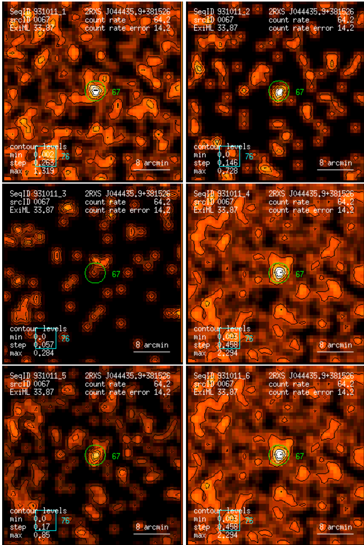
Figure 67: RASS 931011: detection 0067: band rate images, Gaussian filter: (1) PSPC channels 11 – 41, (2) 52 – 90, (3) 91 – 201, (4) 11 – 235, (5) 52 – 201, (6) 11 – 201. Broad band rates in counts/ks. Band rate contour levels in counts/ks/arcmin 2 .
