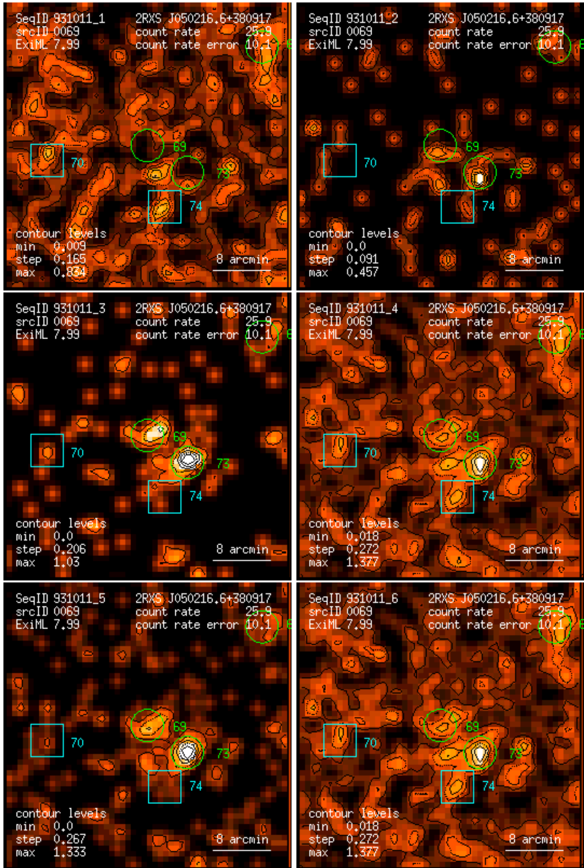
Figure 69: RASS 931011: detection 0069: band rate images, Gaussian filter: (1) PSPC channels 11 – 41, (2) 52 – 90, (3) 91 – 201, (4) 11 – 235, (5) 52 – 201, (6) 11 – 201. Broad band rates in counts/ks. Band rate contour levels in counts/ks/arcmin 2 .
