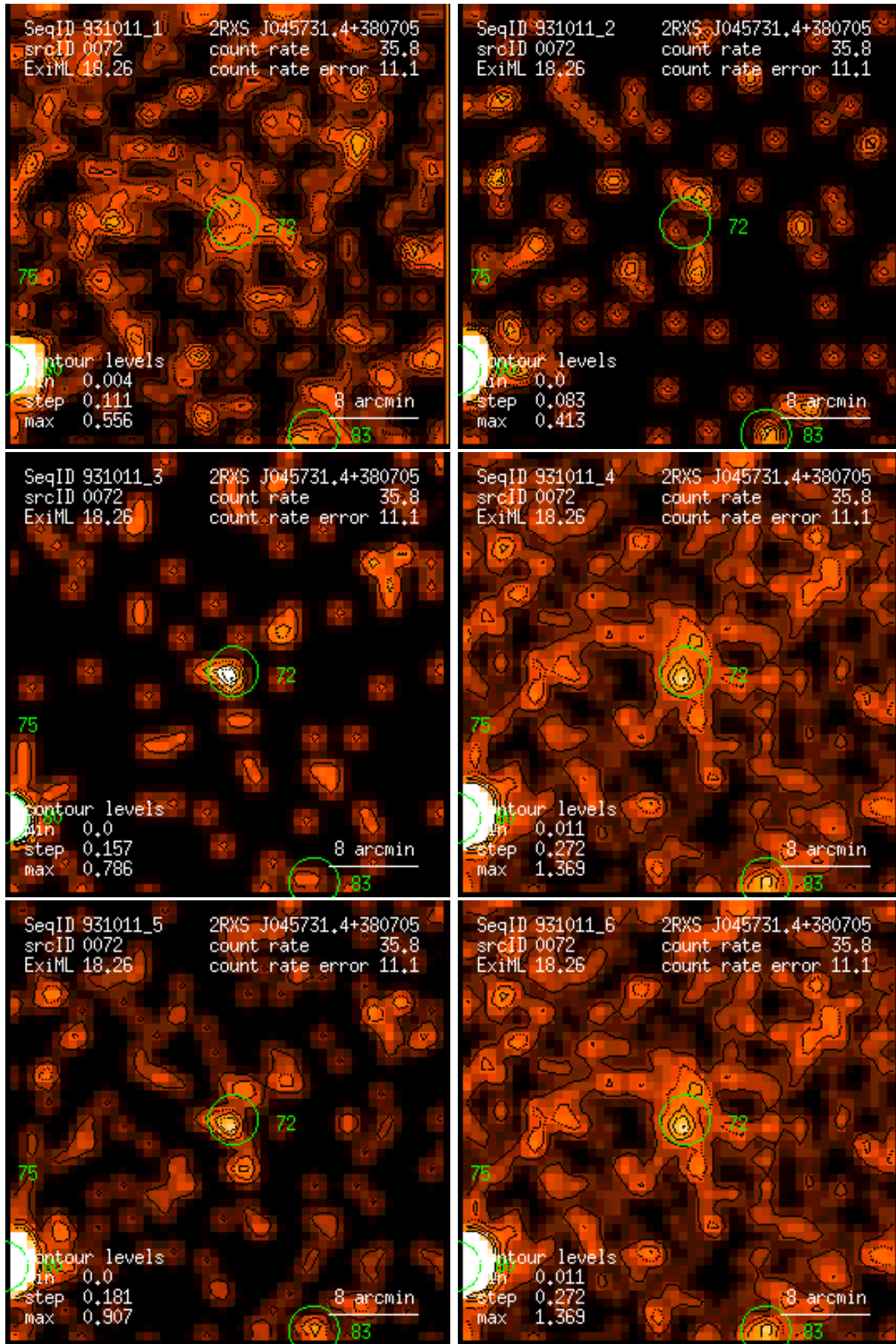
Figure 72: RASS 931011: detection 0072: band rate images, Gaussian filter: (1) PSPC channels 11 – 41, (2) 52 – 90, (3) 91 – 201, (4) 11 – 235, (5) 52 – 201, (6) 11 – 201. Broad band rates in counts/ks. Band rate contour levels in counts/ks/arcmin 2 .
