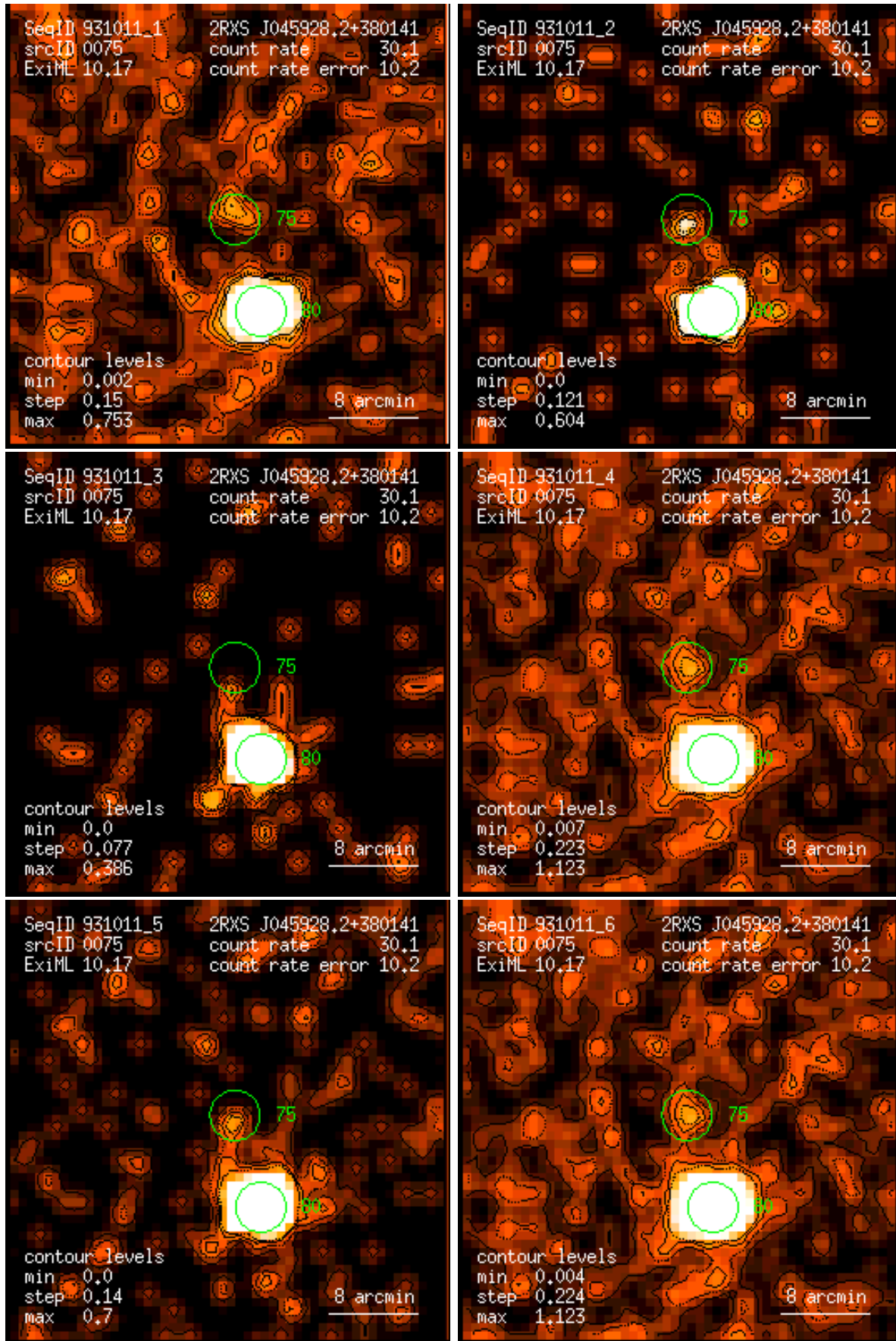
Figure 75: RASS 931011: detection 0075: band rate images, Gaussian filter: (1) PSPC channels 11 – 41, (2) 52 – 90, (3) 91 – 201, (4) 11 – 235, (5) 52 – 201, (6) 11 – 201. Broad band rates in counts/ks. Band rate contour levels in counts/ks/arcmin 2 .
