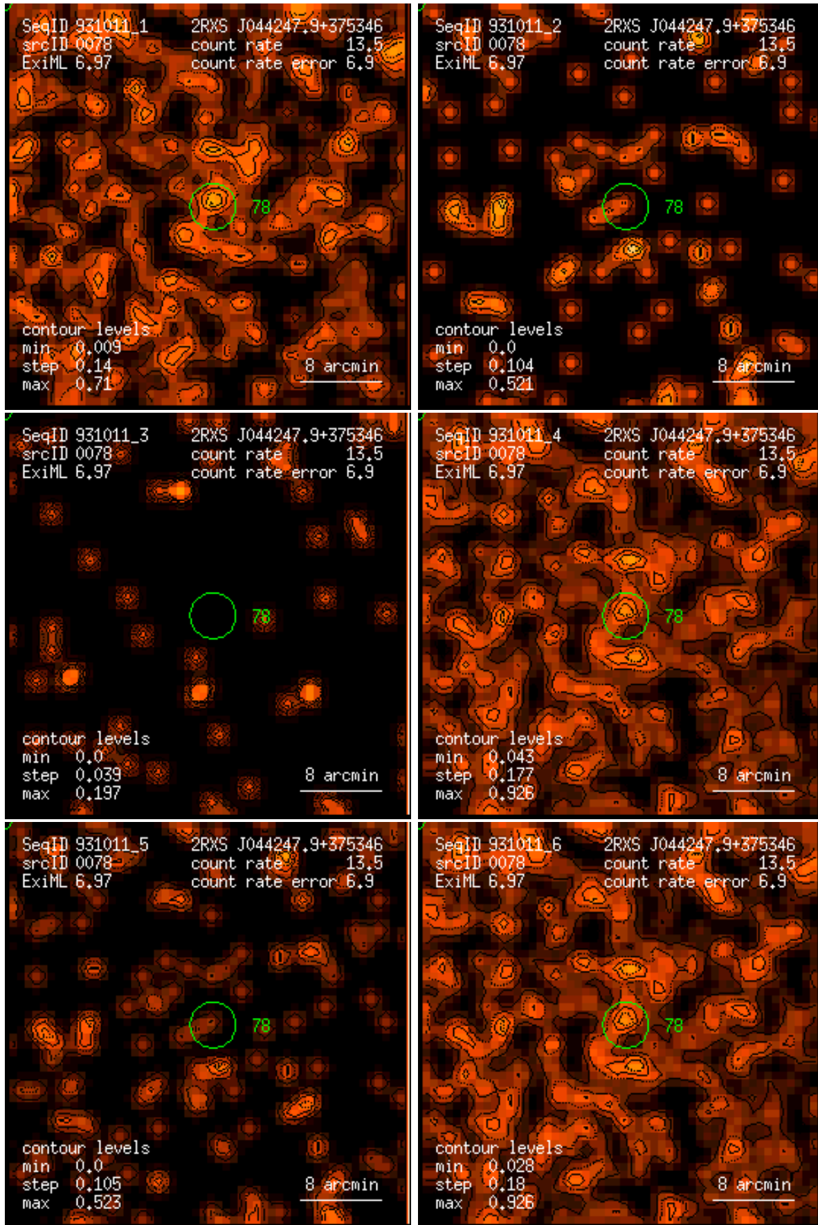
Figure 78: RASS 931011: detection 0078: band rate images, Gaussian filter: (1) PSPC channels 11 – 41, (2) 52 – 90, (3) 91 – 201, (4) 11 – 235, (5) 52 – 201, (6) 11 – 201. Broad band rates in counts/ks. Band rate contour levels in counts/ks/arcmin 2 .
