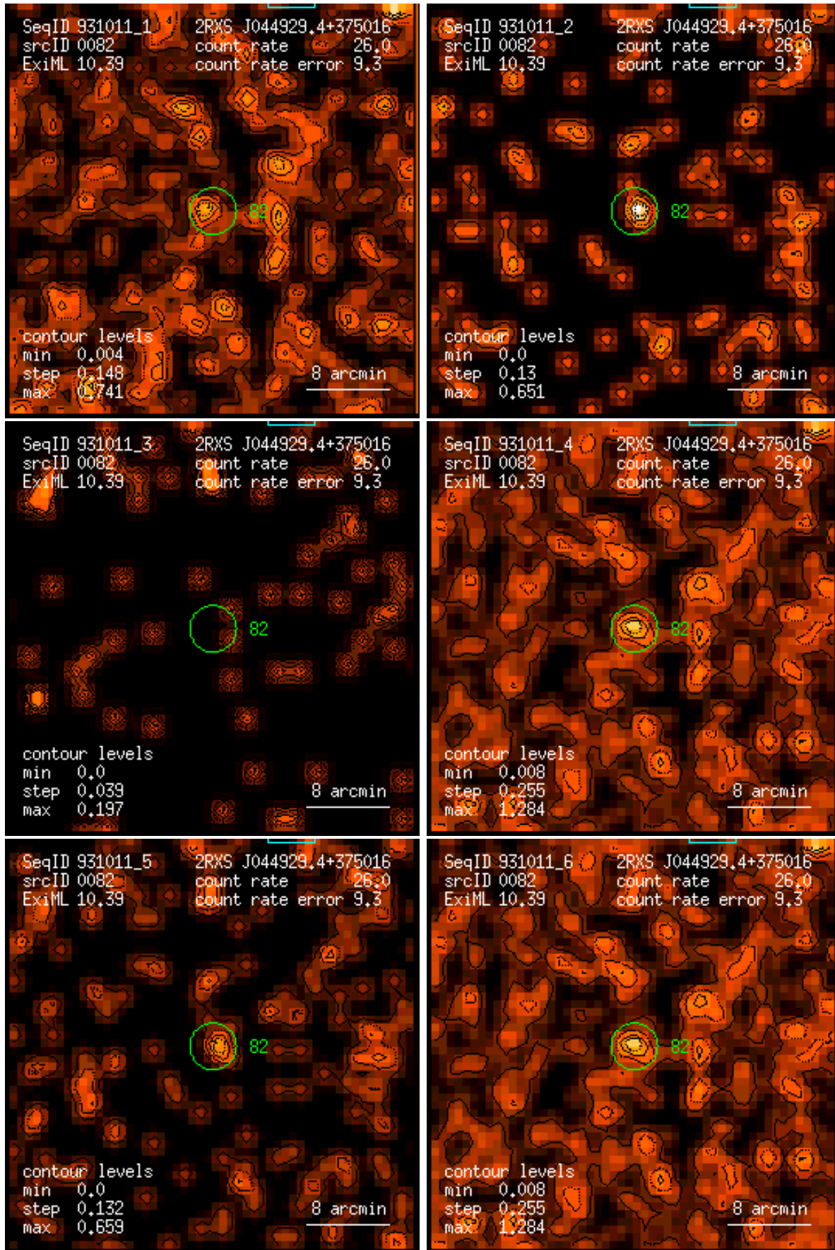
Figure 82: RASS 931011: detection 0082: band rate images, Gaussian filter: (1) PSPC channels 11 – 41, (2) 52 – 90, (3) 91 – 201, (4) 11 – 235, (5) 52 – 201, (6) 11 – 201. Broad band rates in counts/ks. Band rate contour levels in counts/ks/arcmin 2 .
