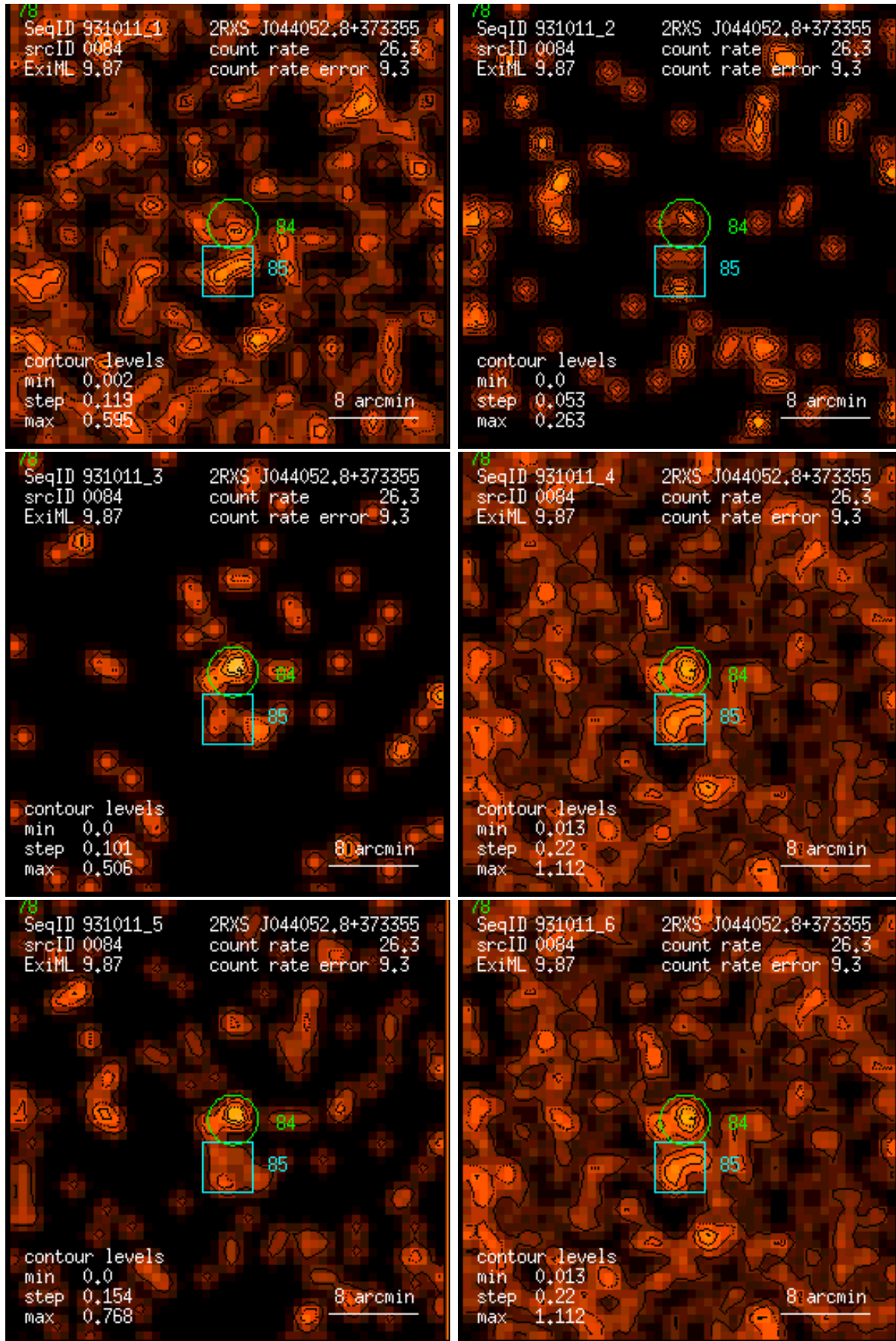
Figure 84: RASS 931011: detection 0084: band rate images, Gaussian filter: (1) PSPC channels 11 – 41, (2) 52 – 90, (3) 91 – 201, (4) 11 – 235, (5) 52 – 201, (6) 11 – 201. Broad band rates in counts/ks. Band rate contour levels in counts/ks/arcmin 2 .
