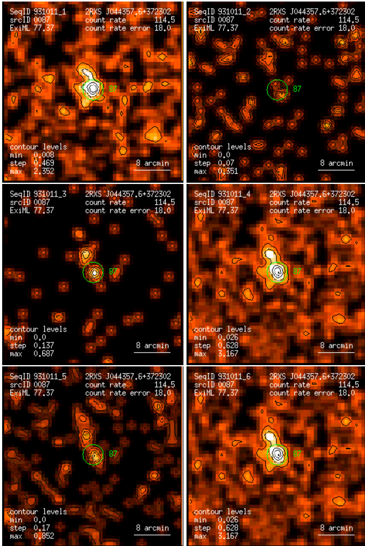
Figure 87: RASS 931011: detection 0087: band rate images, Gaussian filter: (1) PSPC channels 11 – 41, (2) 52 – 90, (3) 91 – 201, (4) 11 – 235, (5) 52 – 201, (6) 11 – 201. Broad band rates in counts/ks. Band rate contour levels in counts/ks/arcmin 2 .
