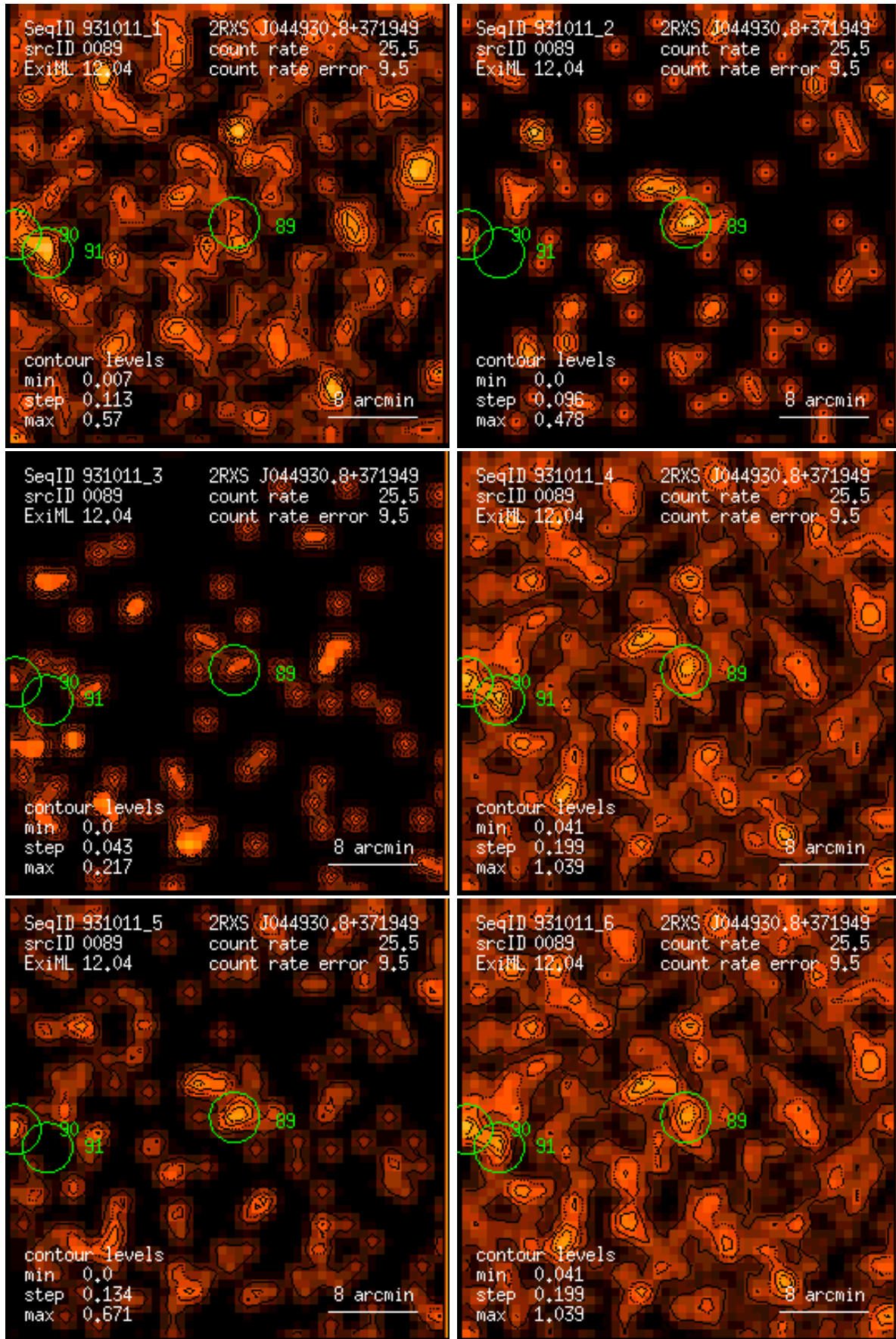
Figure 89: RASS 931011: detection 0089: band rate images, Gaussian filter: (1) PSPC channels 11 – 41, (2) 52 – 90, (3) 91 – 201, (4) 11 – 235, (5) 52 – 201, (6) 11 – 201. Broad band rates in counts/ks. Band rate contour levels in counts/ks/arcmin 2 .
