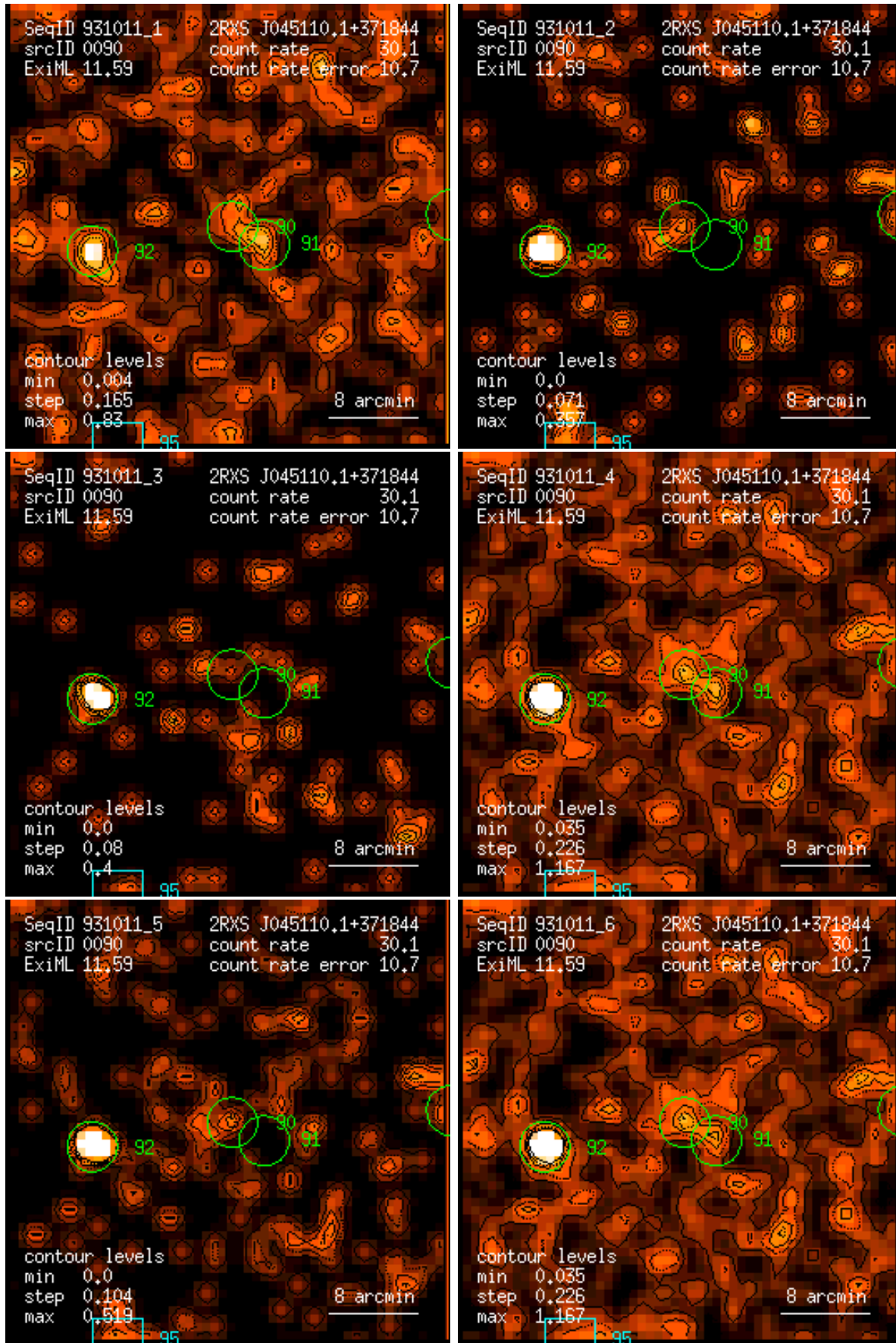
Figure 90: RASS 931011: detection 0090: band rate images, Gaussian filter: (1) PSPC channels 11 – 41, (2) 52 – 90, (3) 91 – 201, (4) 11 – 235, (5) 52 – 201, (6) 11 – 201. Broad band rates in counts/ks. Band rate contour levels in counts/ks/arcmin 2 .
