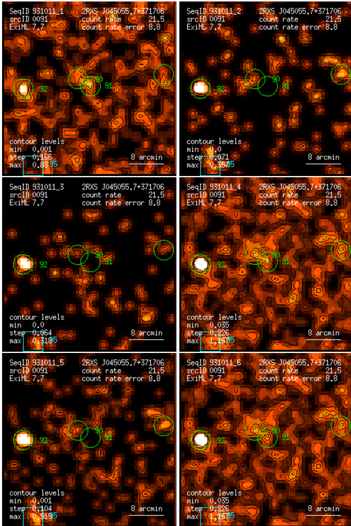
Figure 91: RASS 931011: detection 0091: band rate images, Gaussian filter: (1) PSPC channels 11 – 41, (2) 52 – 90, (3) 91 – 201, (4) 11 – 235, (5) 52 – 201, (6) 11 – 201. Broad band rates in counts/ks. Band rate contour levels in counts/ks/arcmin 2 .
