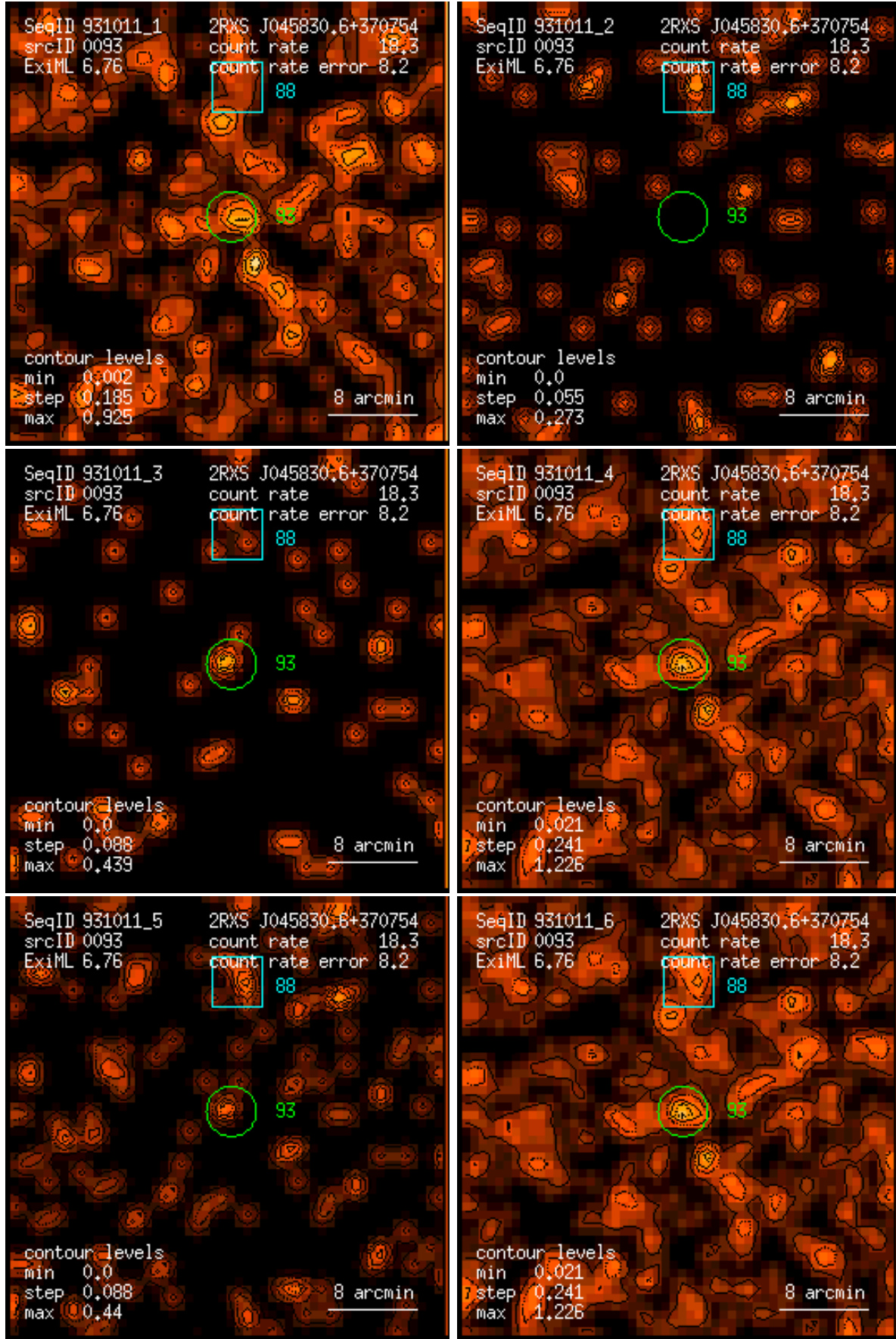
Figure 93: RASS 931011: detection 0093: band rate images, Gaussian filter: (1) PSPC channels 11 – 41, (2) 52 – 90, (3) 91 – 201, (4) 11 – 235, (5) 52 – 201, (6) 11 – 201. Broad band rates in counts/ks. Band rate contour levels in counts/ks/arcmin 2 .
