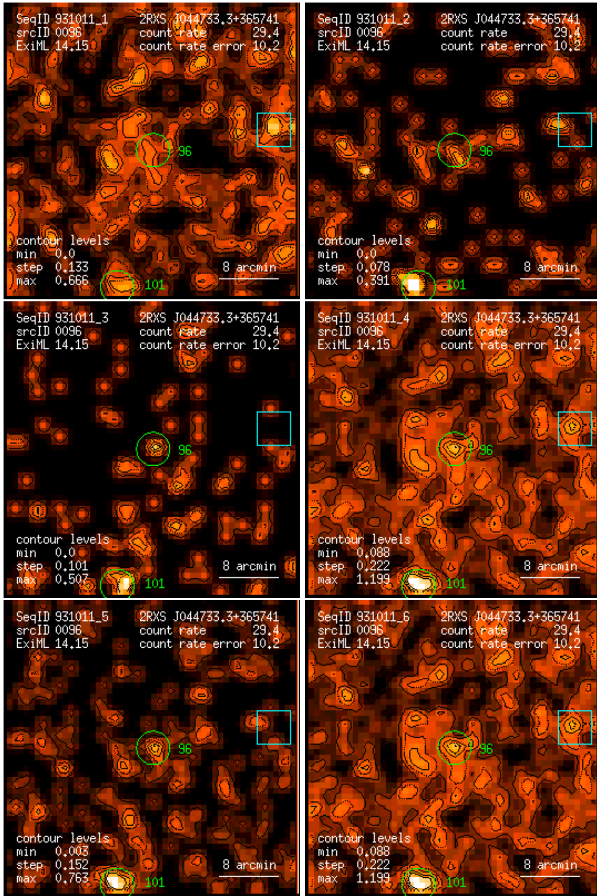
Figure 96: RASS 931011: detection 0096: band rate images, Gaussian filter: (1) PSPC channels 11 – 41, (2) 52 – 90, (3) 91 – 201, (4) 11 – 235, (5) 52 – 201, (6) 11 – 201. Broad band rates in counts/ks. Band rate contour levels in counts/ks/arcmin 2 .
