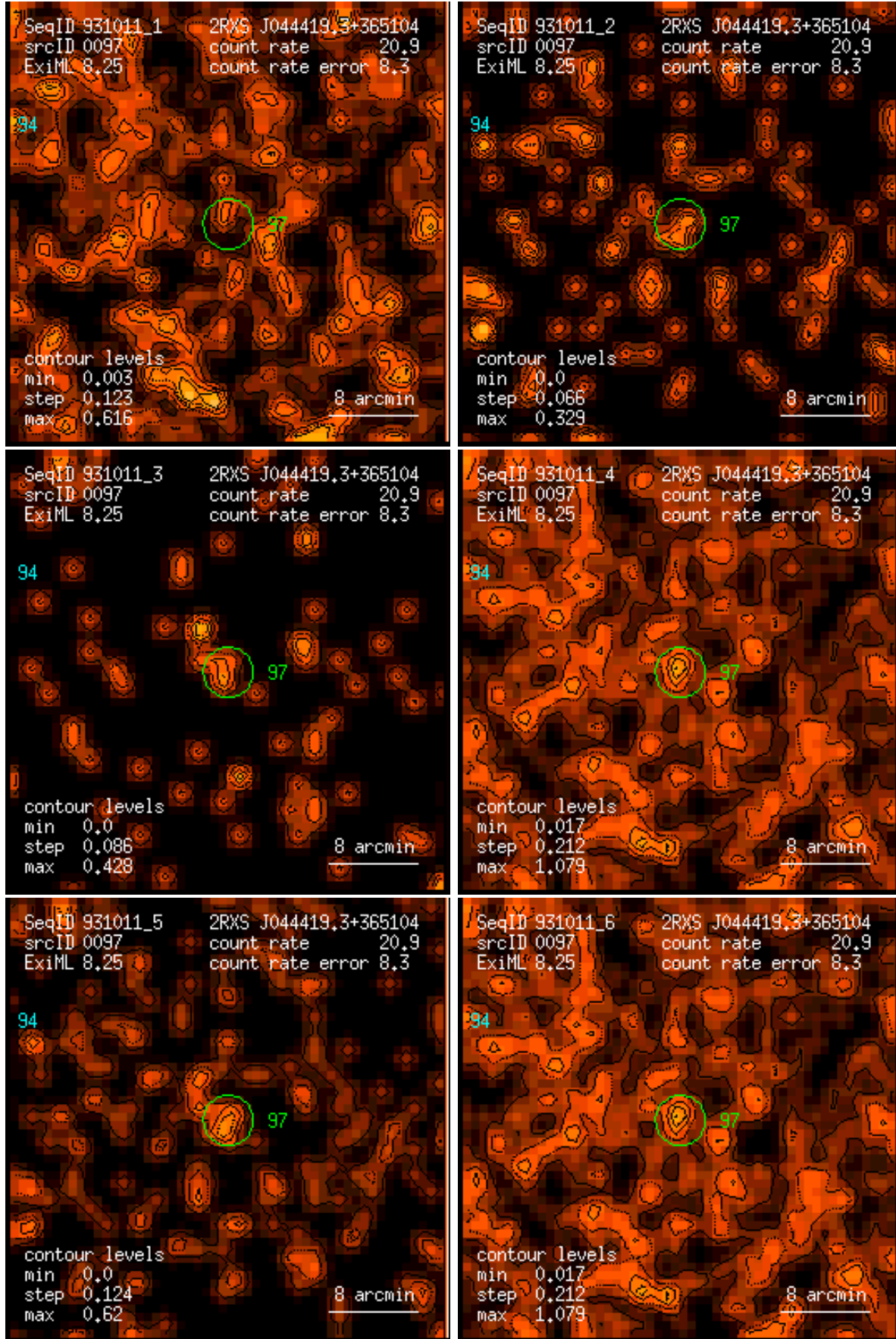
Figure 97: RASS 931011: detection 0097: band rate images, Gaussian filter: (1) PSPC channels 11 – 41, (2) 52 – 90, (3) 91 – 201, (4) 11 – 235, (5) 52 – 201, (6) 11 – 201. Broad band rates in counts/ks. Band rate contour levels in counts/ks/arcmin 2 .
