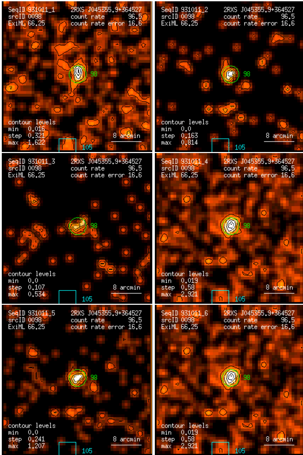
Figure 98: RASS 931011: detection 0098: band rate images, Gaussian filter: (1) PSPC channels 11 – 41, (2) 52 – 90, (3) 91 – 201, (4) 11 – 235, (5) 52 – 201, (6) 11 – 201. Broad band rates in counts/ks. Band rate contour levels in counts/ks/arcmin 2 .
