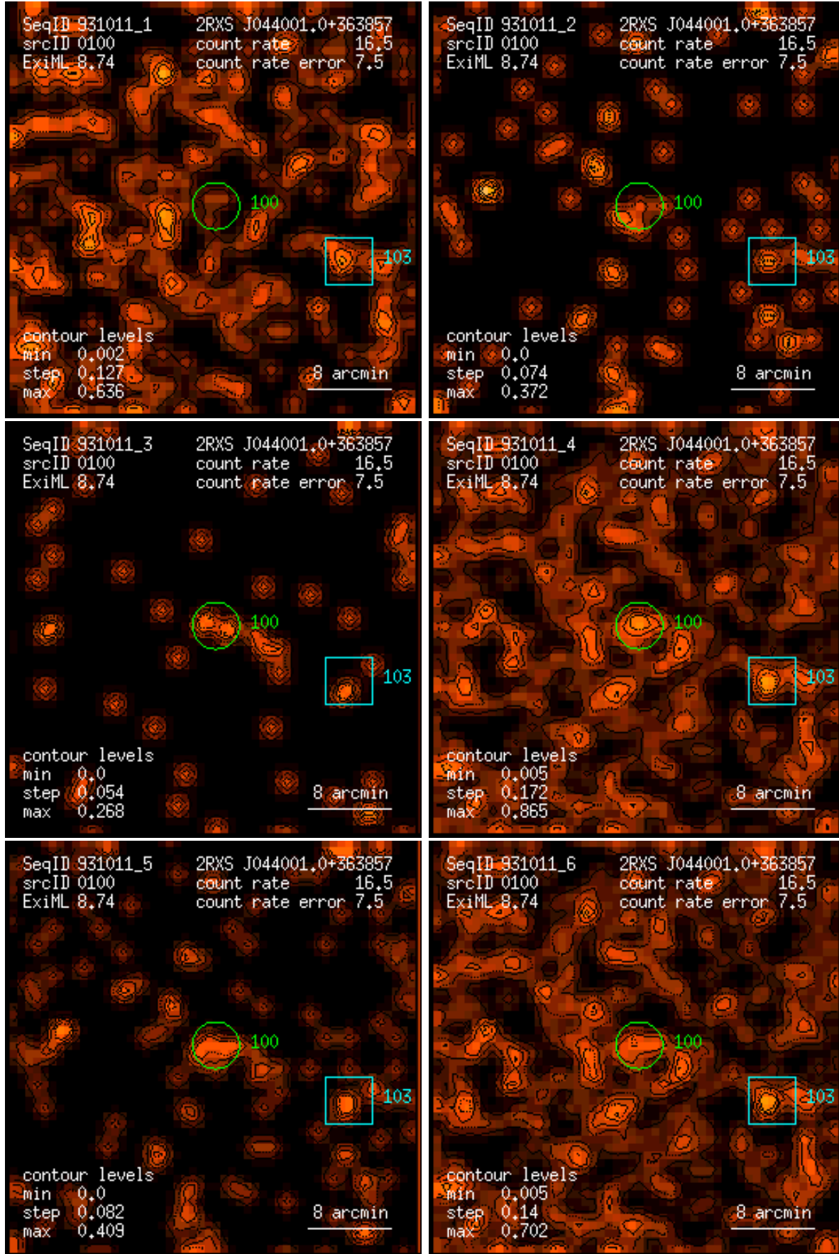
Figure 100: RASS 931011: detection 0100: band rate images, Gaussian filter: (1) PSPC channels 11 – 41, (2) 52 – 90, (3) 91 – 201, (4) 11 – 235, (5) 52 – 201, (6) 11 – 201. Broad band rates in counts/ks. Band rate contour levels in counts/ks/arcmin 2 .
