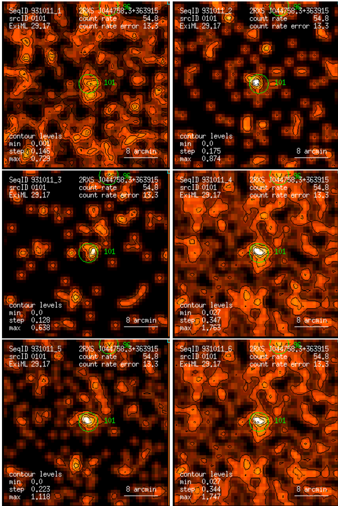
Figure 101: RASS 931011: detection 0101: band rate images, Gaussian filter: (1) PSPC channels 11 – 41, (2) 52 – 90, (3) 91 – 201, (4) 11 – 235, (5) 52 – 201, (6) 11 – 201. Broad band rates in counts/ks. Band rate contour levels in counts/ks/arcmin 2 .
