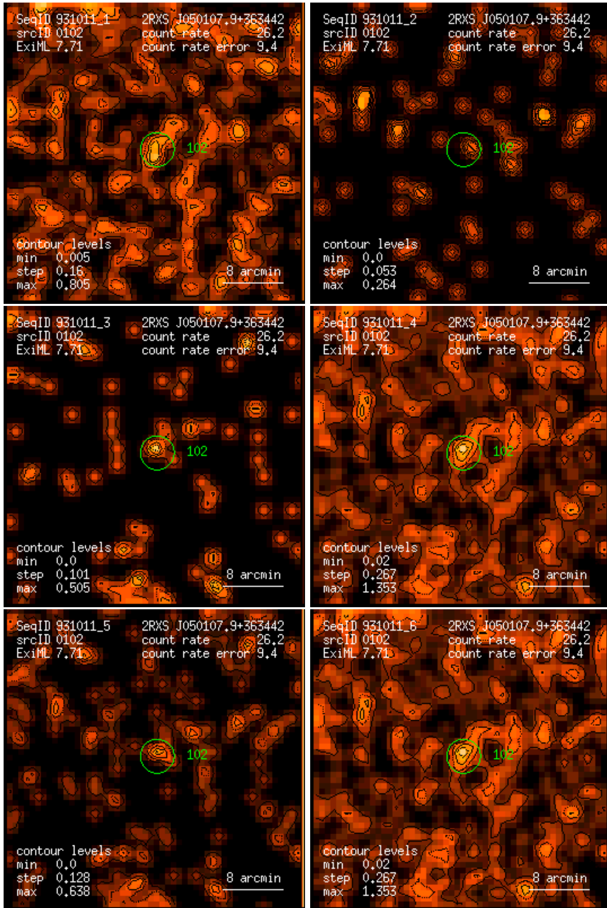
Figure 102: RASS 931011: detection 0102: band rate images, Gaussian filter: (1) PSPC channels 11 – 41, (2) 52 – 90, (3) 91 – 201, (4) 11 – 235, (5) 52 – 201, (6) 11 – 201. Broad band rates in counts/ks. Band rate contour levels in counts/ks/arcmin 2 .
