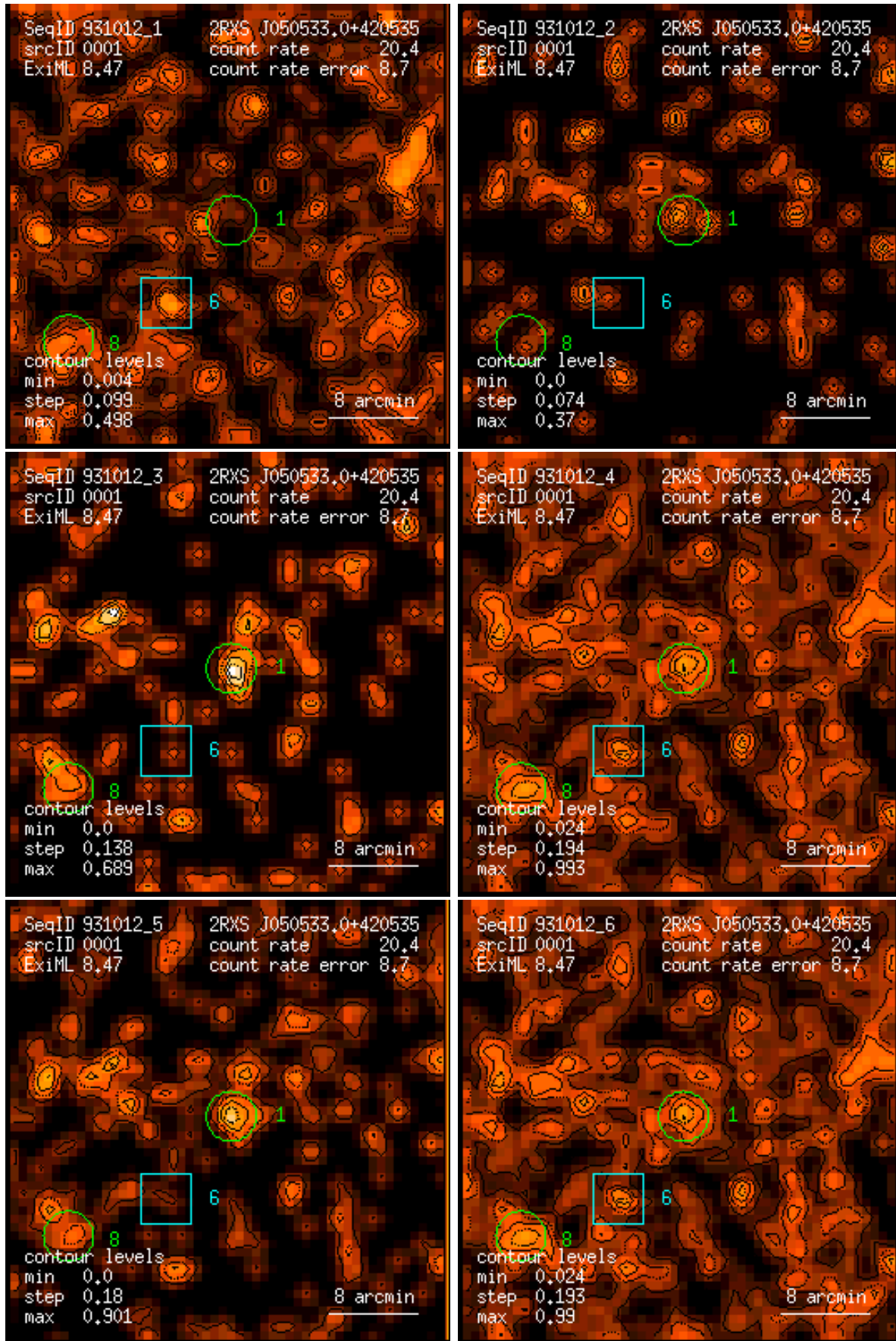
Figure 1: RASS 931012: detection 0001: band rate images, Gaussian filter: (1) PSPC channels 11 – 41, (2) 52 – 90, (3) 91 – 201, (4) 11 – 235, (5) 52 – 201, (6) 11 – 201. Broad band rates in counts/ks. Band rate contour levels in counts/ks/arcmin 2 .
