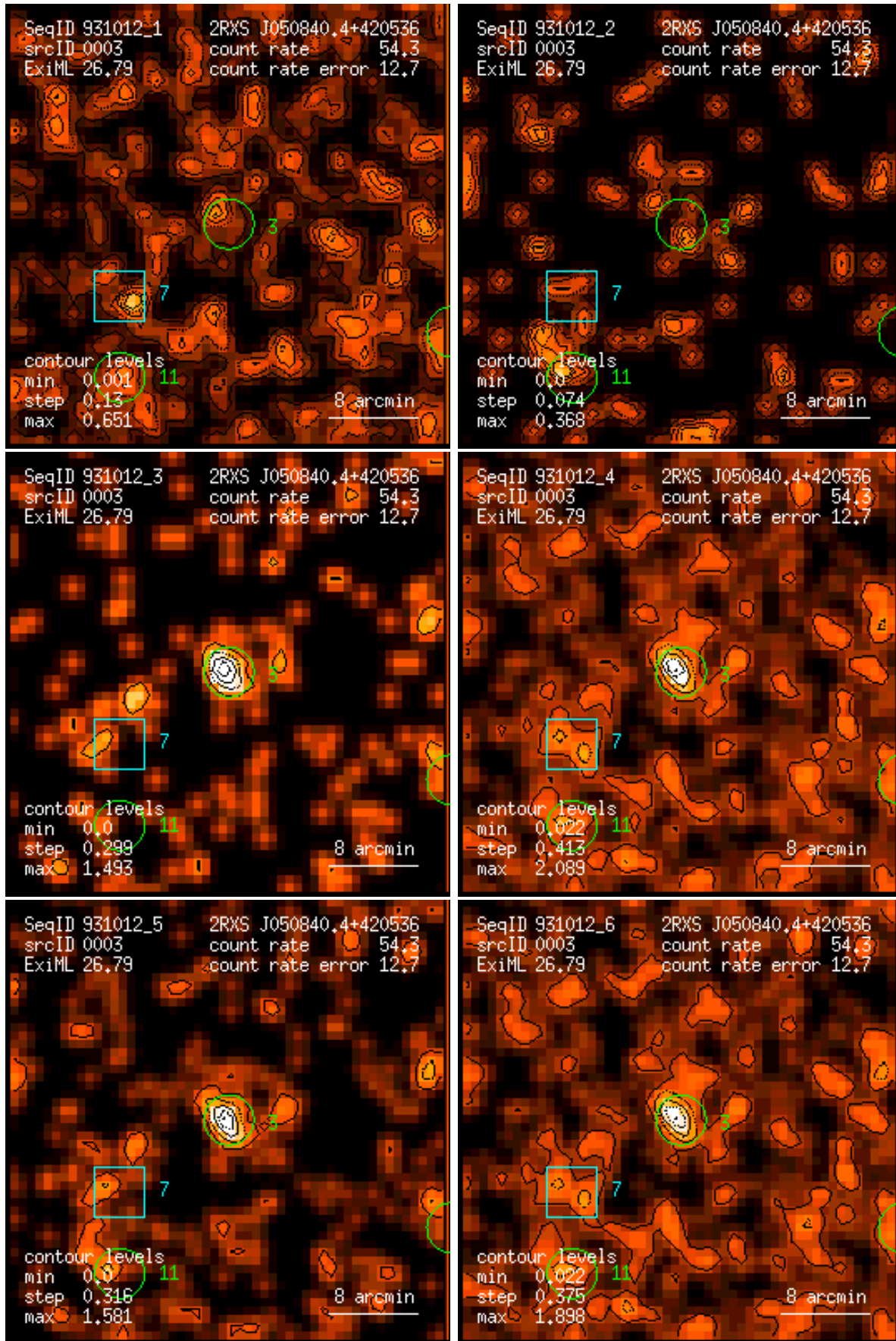
Figure 3: RASS 931012: detection 0003: band rate images, Gaussian filter: (1) PSPC channels 11 – 41, (2) 52 – 90, (3) 91 – 201, (4) 11 – 235, (5) 52 – 201, (6) 11 – 201. Broad band rates in counts/ks. Band rate contour levels in counts/ks/arcmin 2 .
