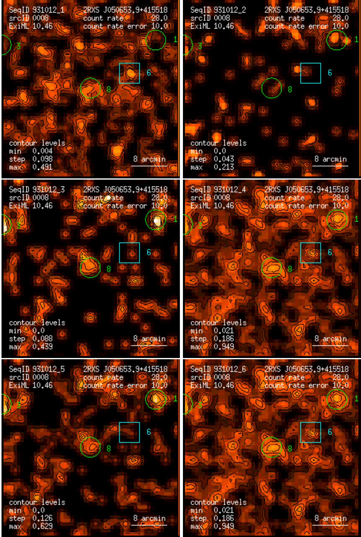
Figure 8: RASS 931012: detection 0008: band rate images, Gaussian filter: (1) PSPC channels 11 – 41, (2) 52 – 90, (3) 91 – 201, (4) 11 – 235, (5) 52 – 201, (6) 11 – 201. Broad band rates in counts/ks. Band rate contour levels in counts/ks/arcmin 2 .
