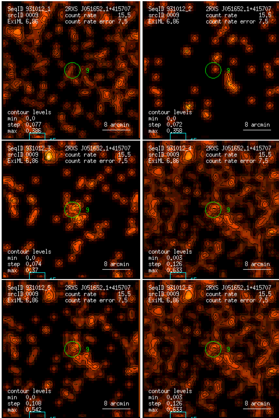
Figure 9: RASS 931012: detection 0009: band rate images, Gaussian filter: (1) PSPC channels 11 – 41, (2) 52 – 90, (3) 91 – 201, (4) 11 – 235, (5) 52 – 201, (6) 11 – 201. Broad band rates in counts/ks. Band rate contour levels in counts/ks/arcmin 2 .
