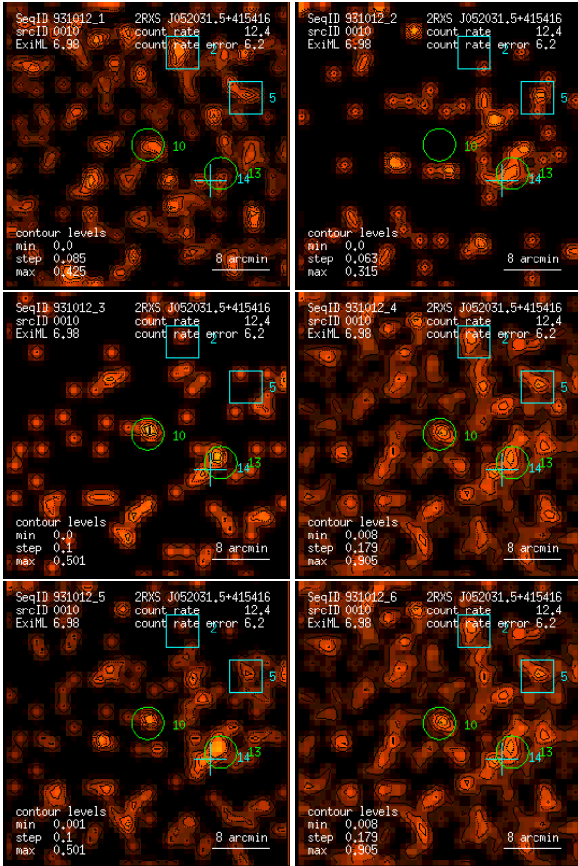
Figure 10: RASS 931012: detection 0010: band rate images, Gaussian filter: (1) PSPC channels 11 – 41, (2) 52 – 90, (3) 91 – 201, (4) 11 – 235, (5) 52 – 201, (6) 11 – 201. Broad band rates in counts/ks. Band rate contour levels in counts/ks/arcmin 2 .
