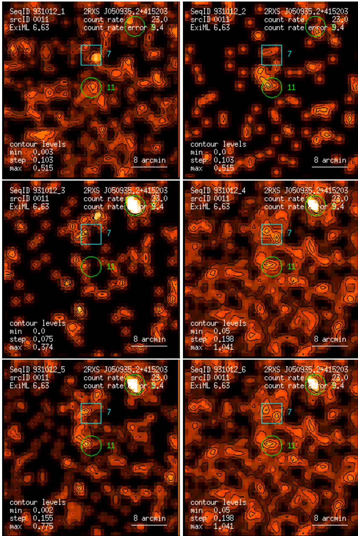
Figure 11: RASS 931012: detection 0011: band rate images, Gaussian filter: (1) PSPC channels 11 – 41, (2) 52 – 90, (3) 91 – 201, (4) 11 – 235, (5) 52 – 201, (6) 11 – 201. Broad band rates in counts/ks. Band rate contour levels in counts/ks/arcmin 2 .
