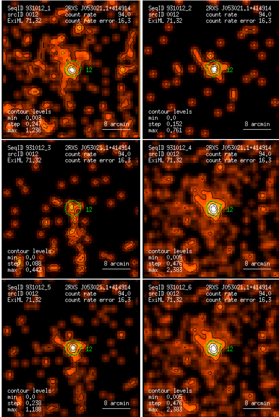
Figure 12: RASS 931012: detection 0012: band rate images, Gaussian filter: (1) PSPC channels 11 – 41, (2) 52 – 90, (3) 91 – 201, (4) 11 – 235, (5) 52 – 201, (6) 11 – 201. Broad band rates in counts/ks. Band rate contour levels in counts/ks/arcmin 2 .
