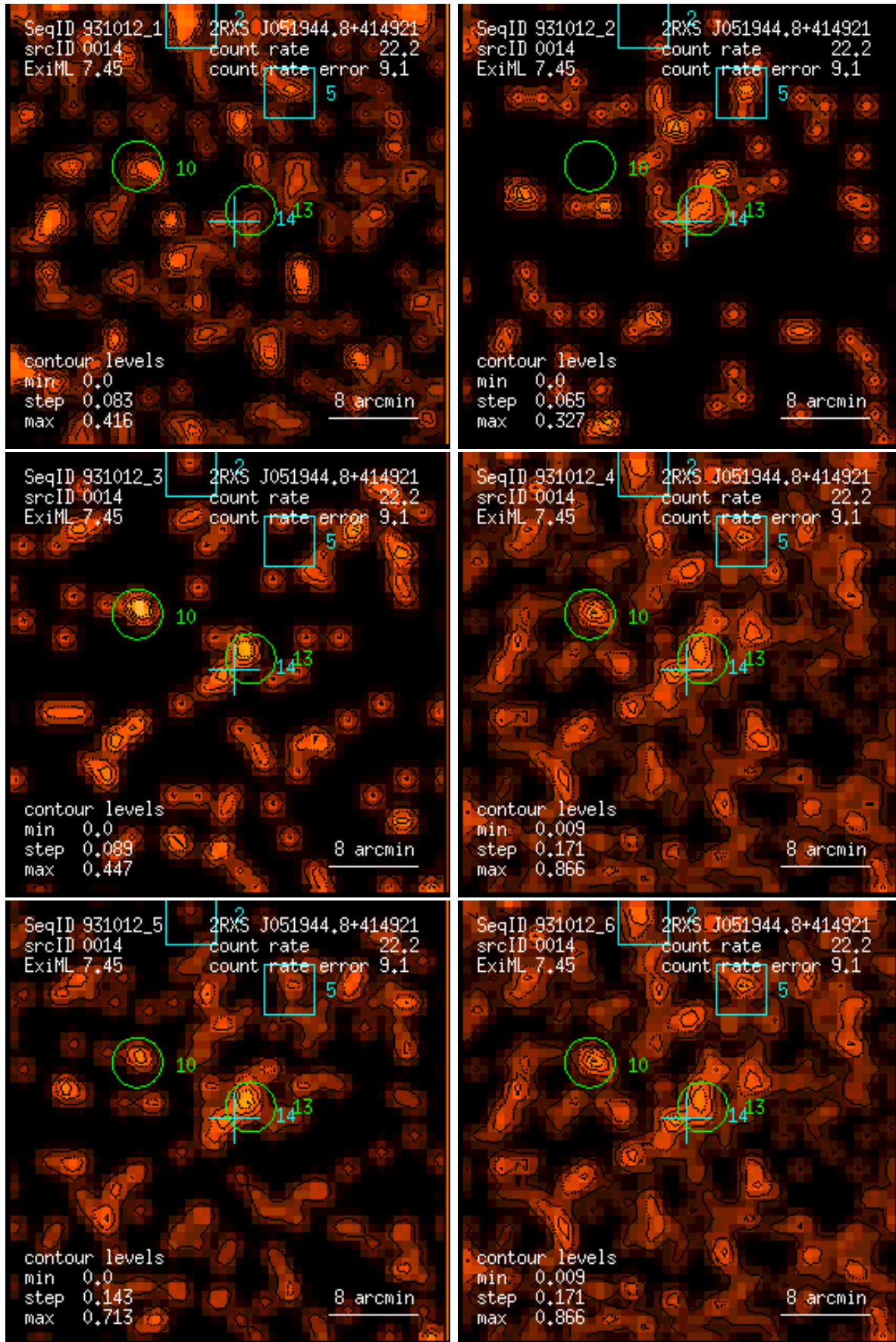
Figure 14: RASS 931012: detection 0014: band rate images, Gaussian filter: (1) PSPC channels 11 – 41, (2) 52 – 90, (3) 91 – 201, (4) 11 – 235, (5) 52 – 201, (6) 11 – 201. Broad band rates in counts/ks. Band rate contour levels in counts/ks/arcmin 2 .
