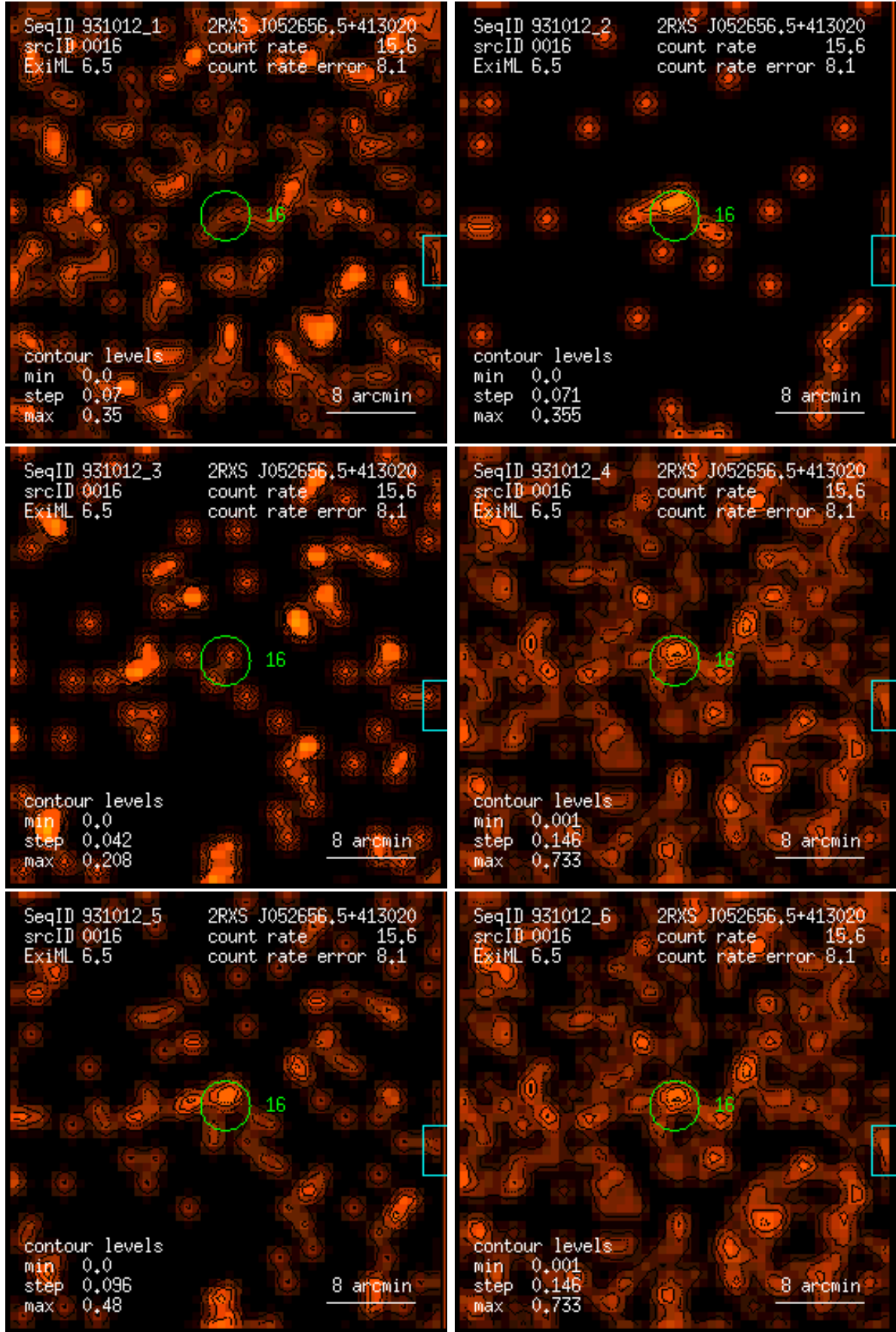
Figure 16: RASS 931012: detection 0016: band rate images, Gaussian filter: (1) PSPC channels 11 – 41, (2) 52 – 90, (3) 91 – 201, (4) 11 – 235, (5) 52 – 201, (6) 11 – 201. Broad band rates in counts/ks. Band rate contour levels in counts/ks/arcmin 2 .
