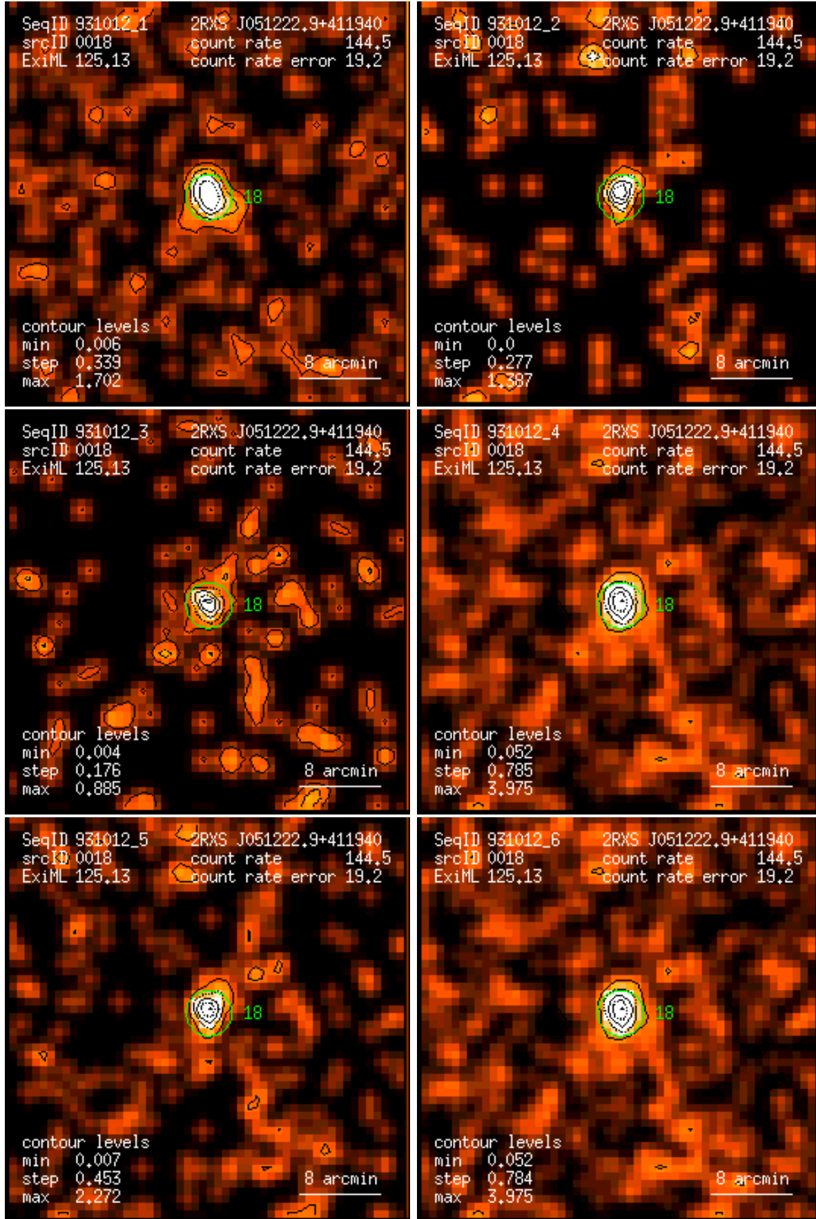
Figure 18: RASS 931012: detection 0018: band rate images, Gaussian filter: (1) PSPC channels 11 – 41, (2) 52 – 90, (3) 91 – 201, (4) 11 – 235, (5) 52 – 201, (6) 11 – 201. Broad band rates in counts/ks. Band rate contour levels in counts/ks/arcmin 2 .
