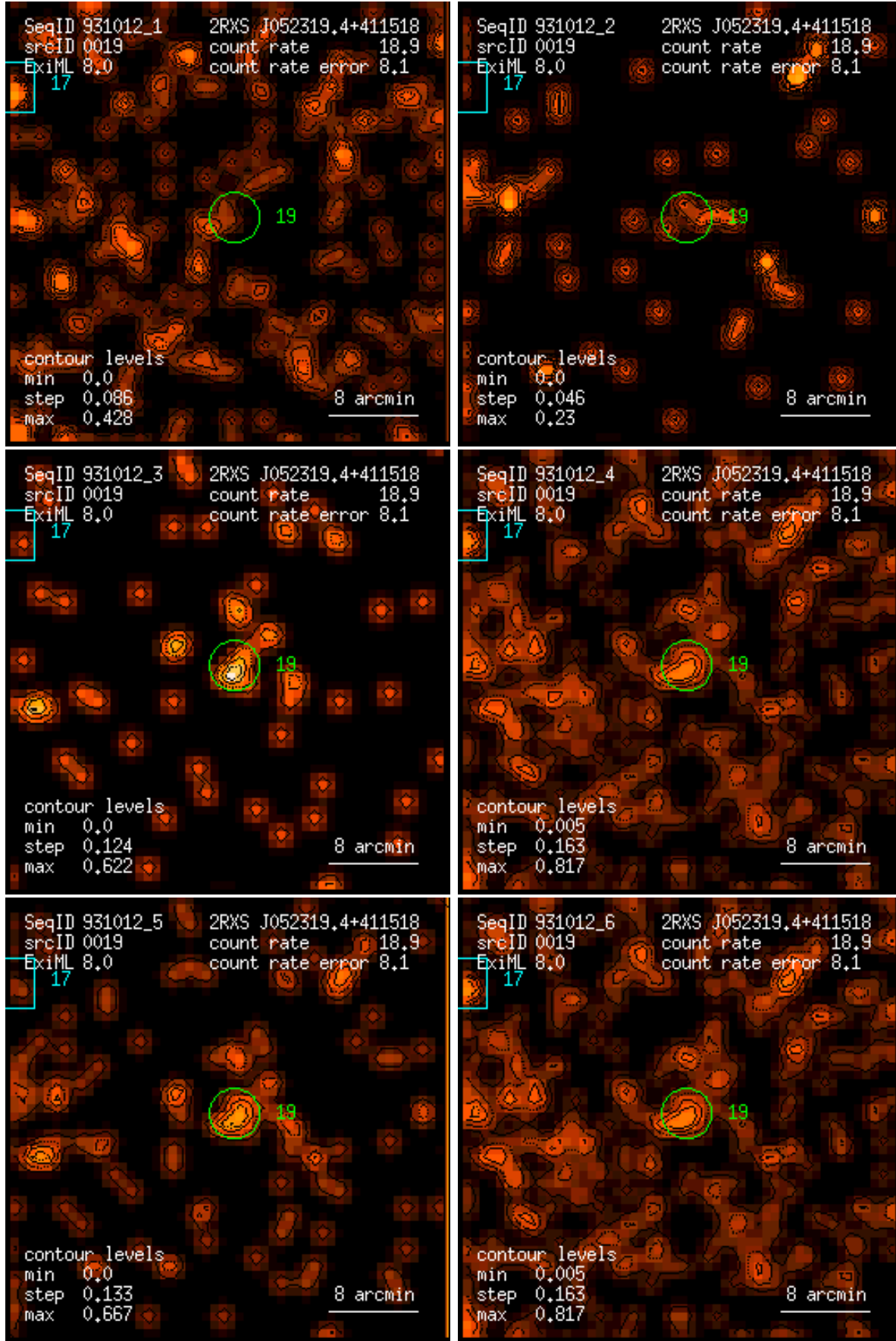
Figure 19: RASS 931012: detection 0019: band rate images, Gaussian filter: (1) PSPC channels 11 – 41, (2) 52 – 90, (3) 91 – 201, (4) 11 – 235, (5) 52 – 201, (6) 11 – 201. Broad band rates in counts/ks. Band rate contour levels in counts/ks/arcmin 2 .
