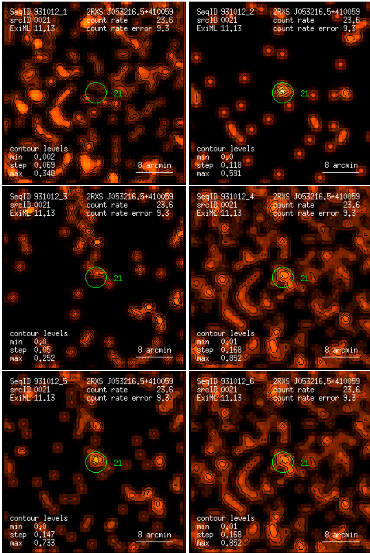
Figure 21: RASS 931012: detection 0021: band rate images, Gaussian filter: (1) PSPC channels 11 – 41, (2) 52 – 90, (3) 91 – 201, (4) 11 – 235, (5) 52 – 201, (6) 11 – 201. Broad band rates in counts/ks. Band rate contour levels in counts/ks/arcmin 2 .
