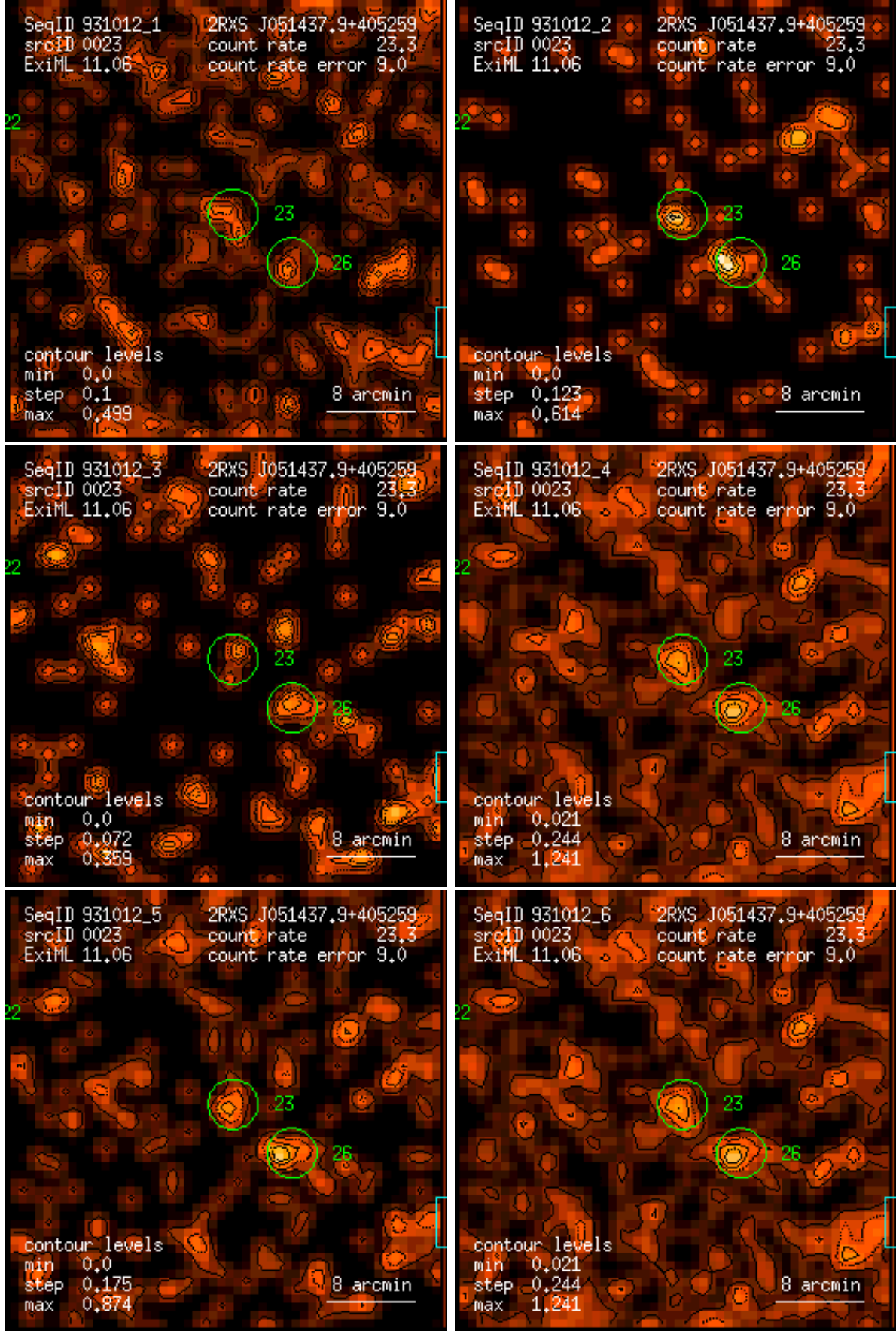
Figure 23: RASS 931012: detection 0023: band rate images, Gaussian filter: (1) PSPC channels 11 – 41, (2) 52 – 90, (3) 91 – 201, (4) 11 – 235, (5) 52 – 201, (6) 11 – 201. Broad band rates in counts/ks. Band rate contour levels in counts/ks/arcmin 2 .
