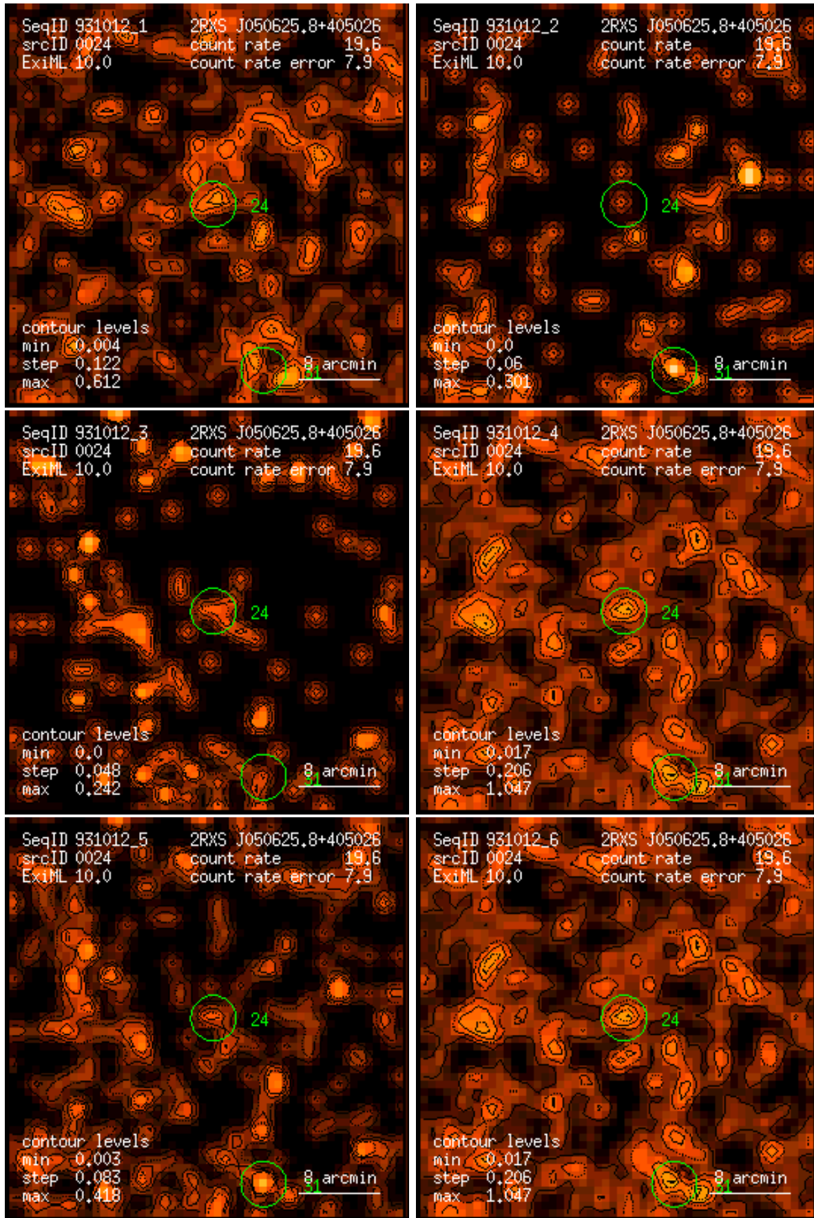
Figure 24: RASS 931012: detection 0024: band rate images, Gaussian filter: (1) PSPC channels 11 – 41, (2) 52 – 90, (3) 91 – 201, (4) 11 – 235, (5) 52 – 201, (6) 11 – 201. Broad band rates in counts/ks. Band rate contour levels in counts/ks/arcmin 2 .
