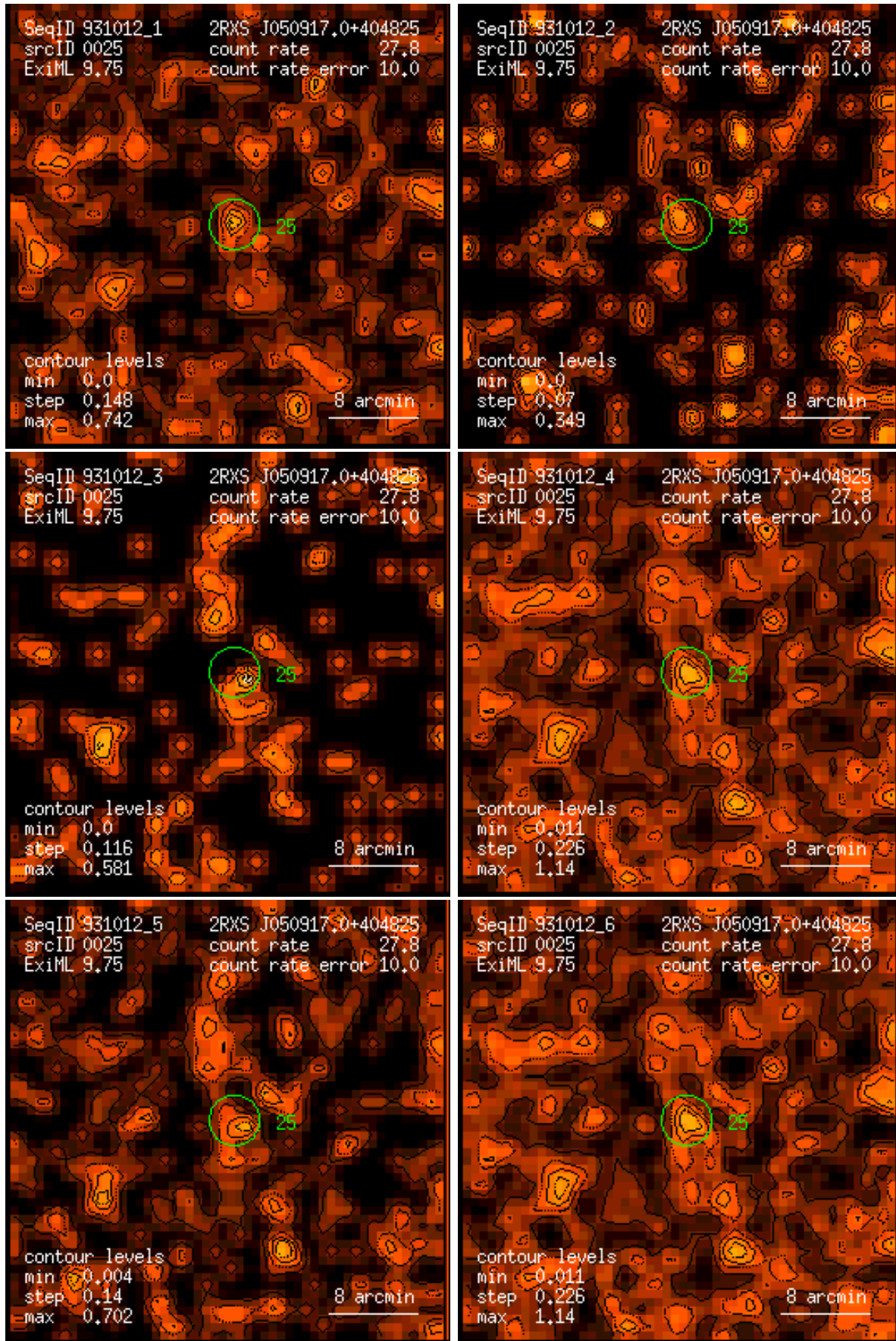
Figure 25: RASS 931012: detection 0025: band rate images, Gaussian filter: (1) PSPC channels 11 – 41, (2) 52 – 90, (3) 91 – 201, (4) 11 – 235, (5) 52 – 201, (6) 11 – 201. Broad band rates in counts/ks. Band rate contour levels in counts/ks/arcmin 2 .
