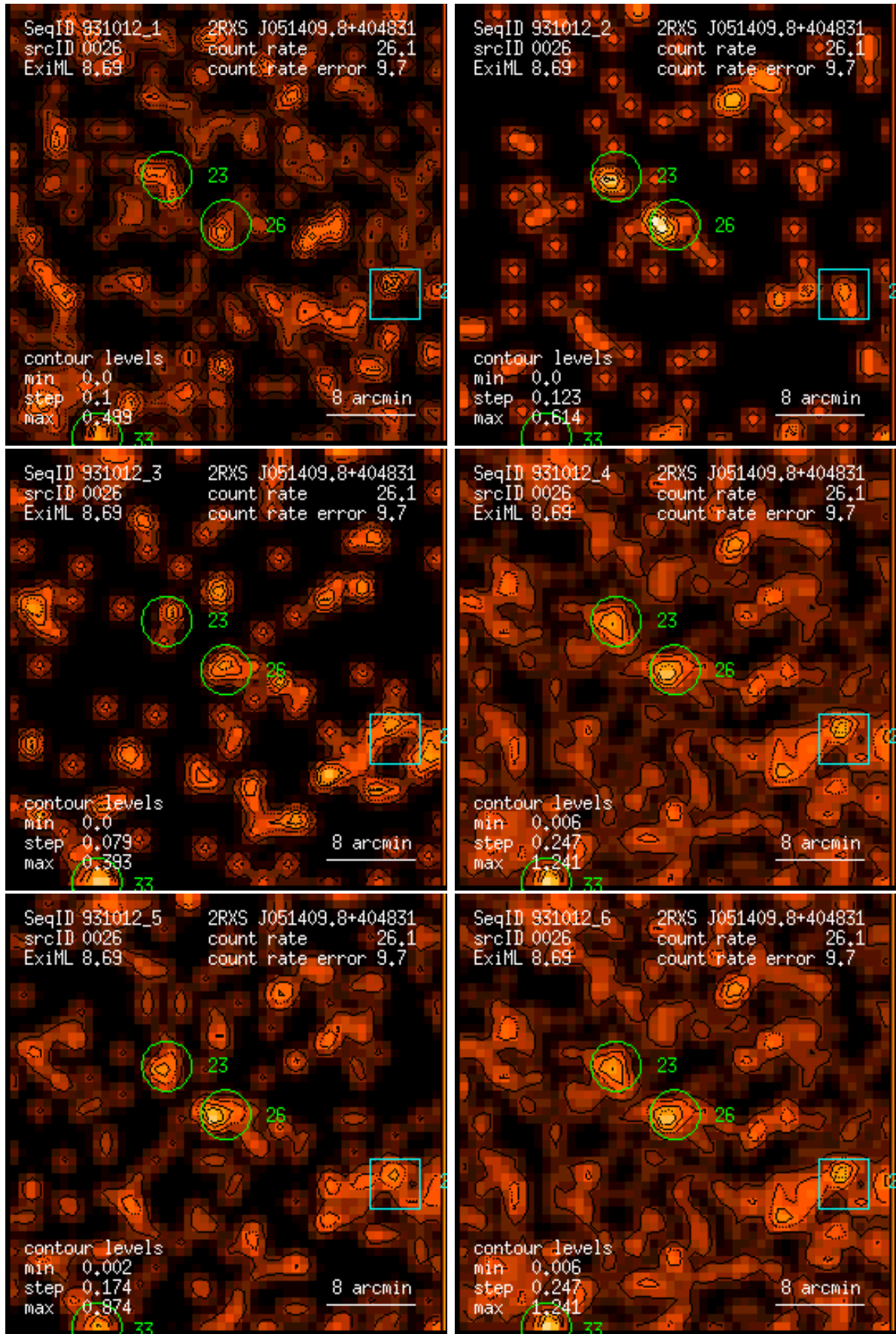
Figure 26: RASS 931012: detection 0026: band rate images, Gaussian filter: (1) PSPC channels 11 – 41, (2) 52 – 90, (3) 91 – 201, (4) 11 – 235, (5) 52 – 201, (6) 11 – 201. Broad band rates in counts/ks. Band rate contour levels in counts/ks/arcmin 2 .
