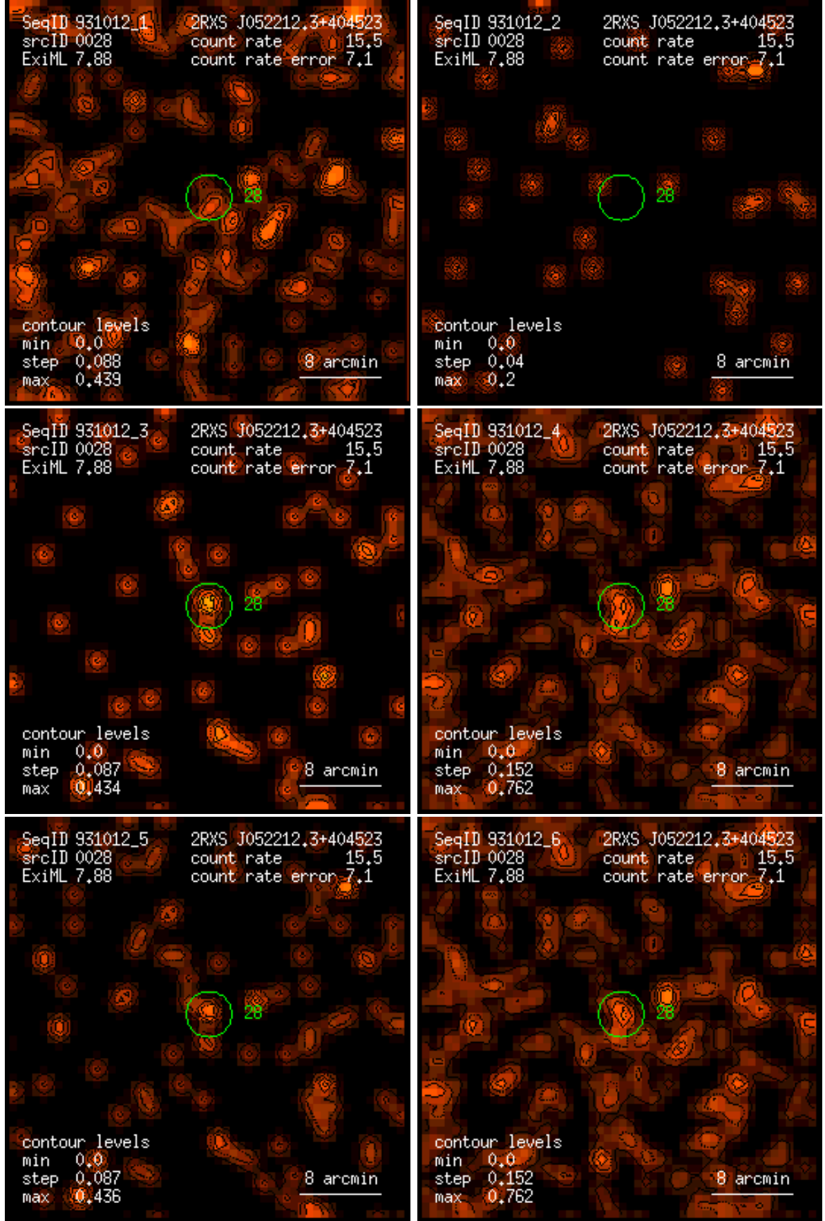
Figure 28: RASS 931012: detection 0028: band rate images, Gaussian filter: (1) PSPC channels 11 – 41, (2) 52 – 90, (3) 91 – 201, (4) 11 – 235, (5) 52 – 201, (6) 11 – 201. Broad band rates in counts/ks. Band rate contour levels in counts/ks/arcmin 2 .
