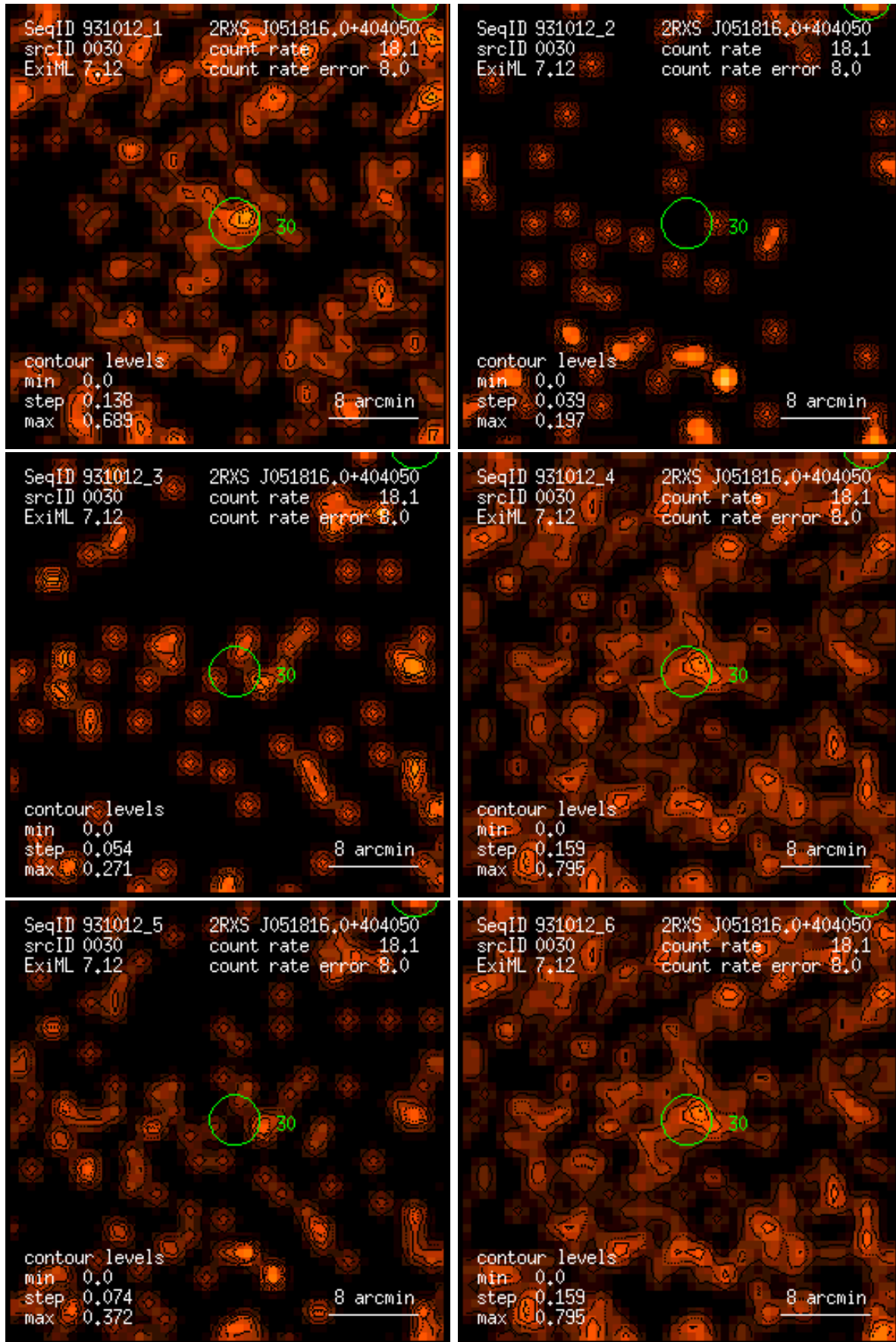
Figure 30: RASS 931012: detection 0030: band rate images, Gaussian filter: (1) PSPC channels 11 – 41, (2) 52 – 90, (3) 91 – 201, (4) 11 – 235, (5) 52 – 201, (6) 11 – 201. Broad band rates in counts/ks. Band rate contour levels in counts/ks/arcmin 2 .
