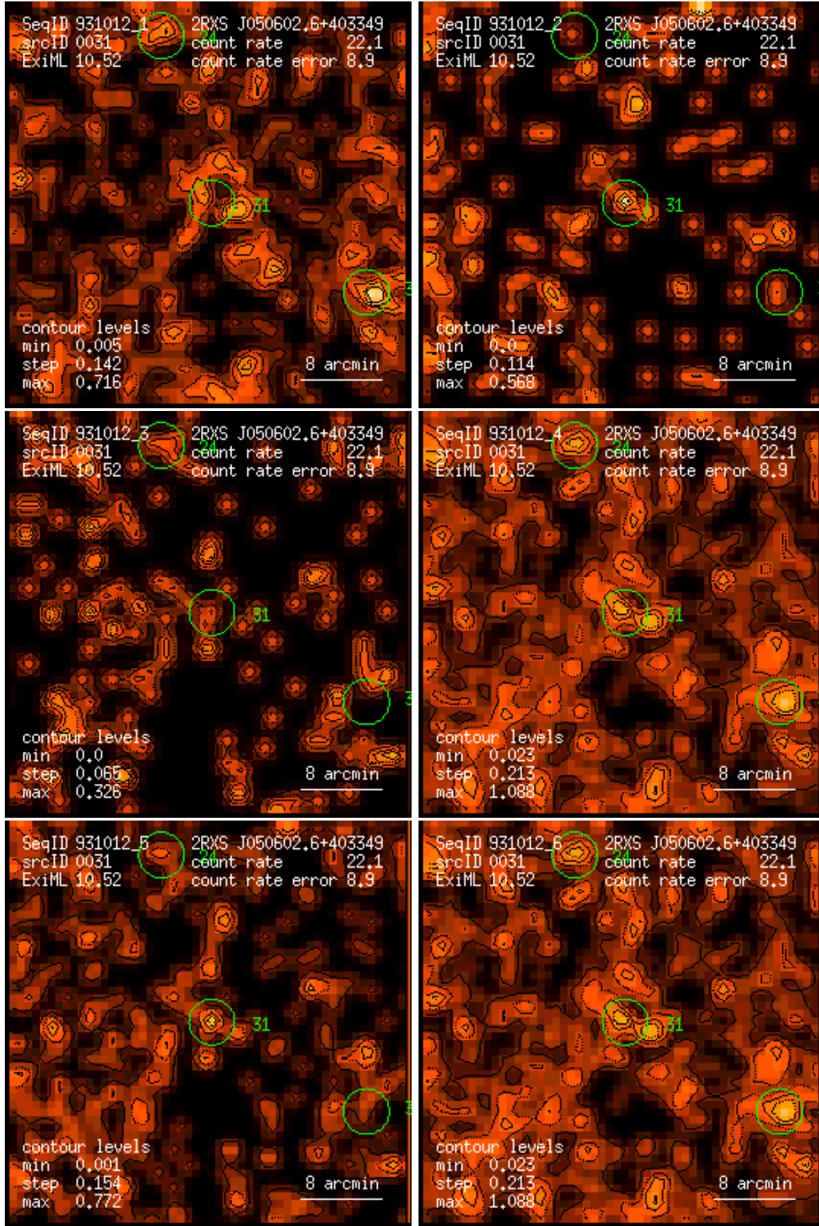
Figure 31: RASS 931012: detection 0031: band rate images, Gaussian filter: (1) PSPC channels 11 – 41, (2) 52 – 90, (3) 91 – 201, (4) 11 – 235, (5) 52 – 201, (6) 11 – 201. Broad band rates in counts/ks. Band rate contour levels in counts/ks/arcmin 2 .
