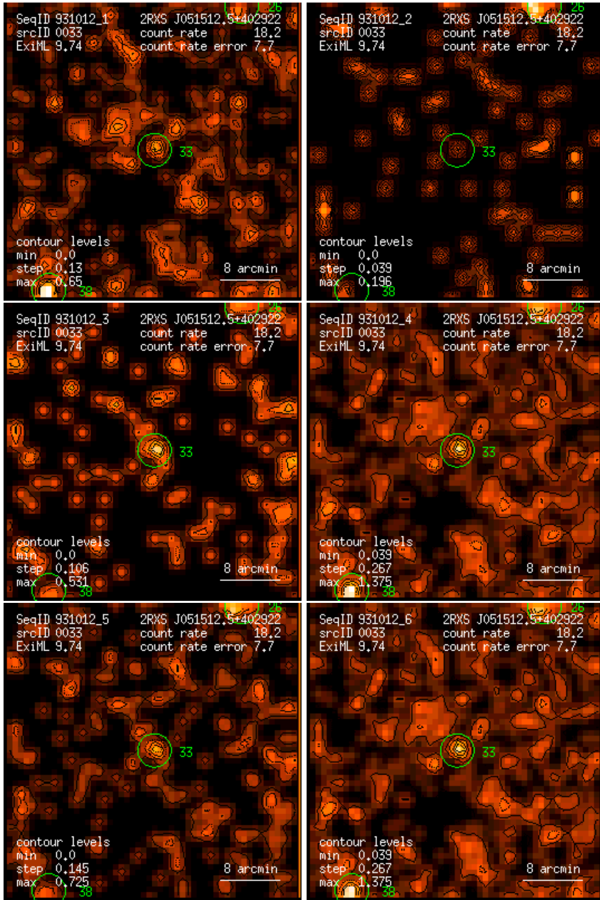
Figure 33: RASS 931012: detection 0033: band rate images, Gaussian filter: (1) PSPC channels 11 – 41, (2) 52 – 90, (3) 91 – 201, (4) 11 – 235, (5) 52 – 201, (6) 11 – 201. Broad band rates in counts/ks. Band rate contour levels in counts/ks/arcmin 2 .
