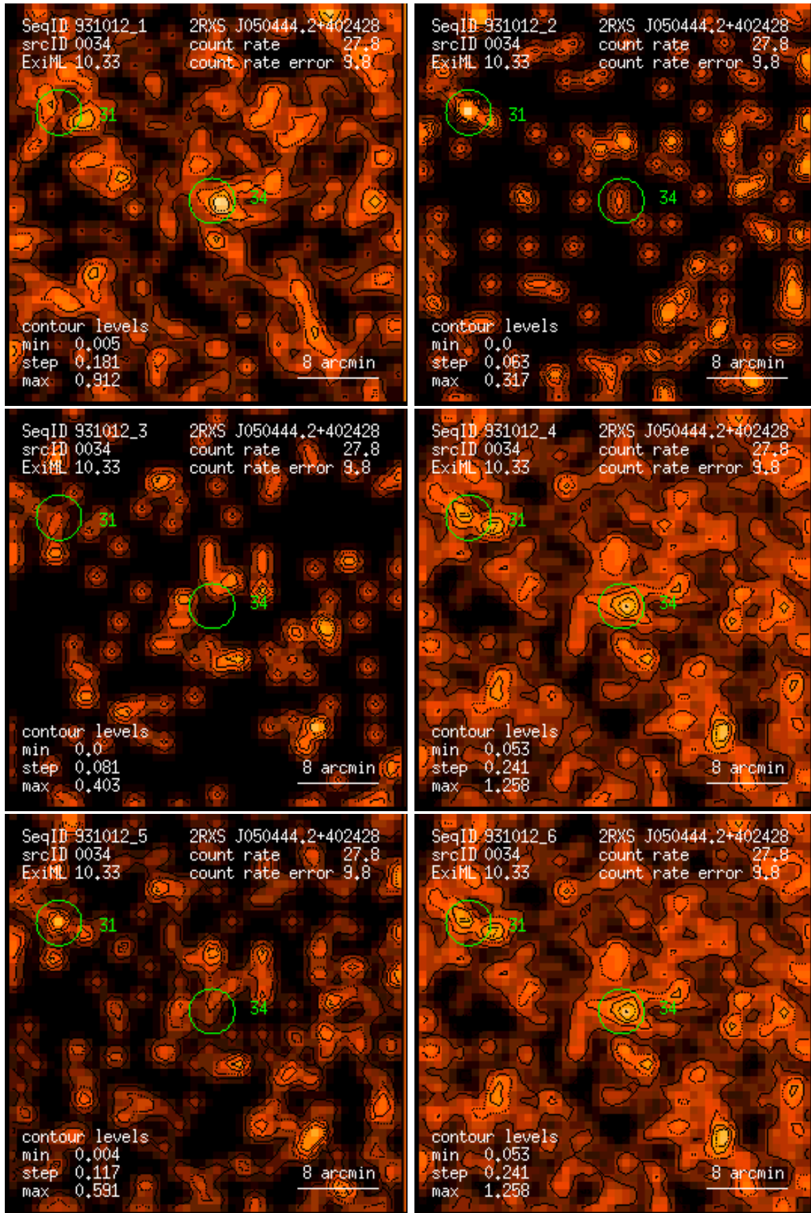
Figure 34: RASS 931012: detection 0034: band rate images, Gaussian filter: (1) PSPC channels 11 – 41, (2) 52 – 90, (3) 91 – 201, (4) 11 – 235, (5) 52 – 201, (6) 11 – 201. Broad band rates in counts/ks. Band rate contour levels in counts/ks/arcmin 2 .
