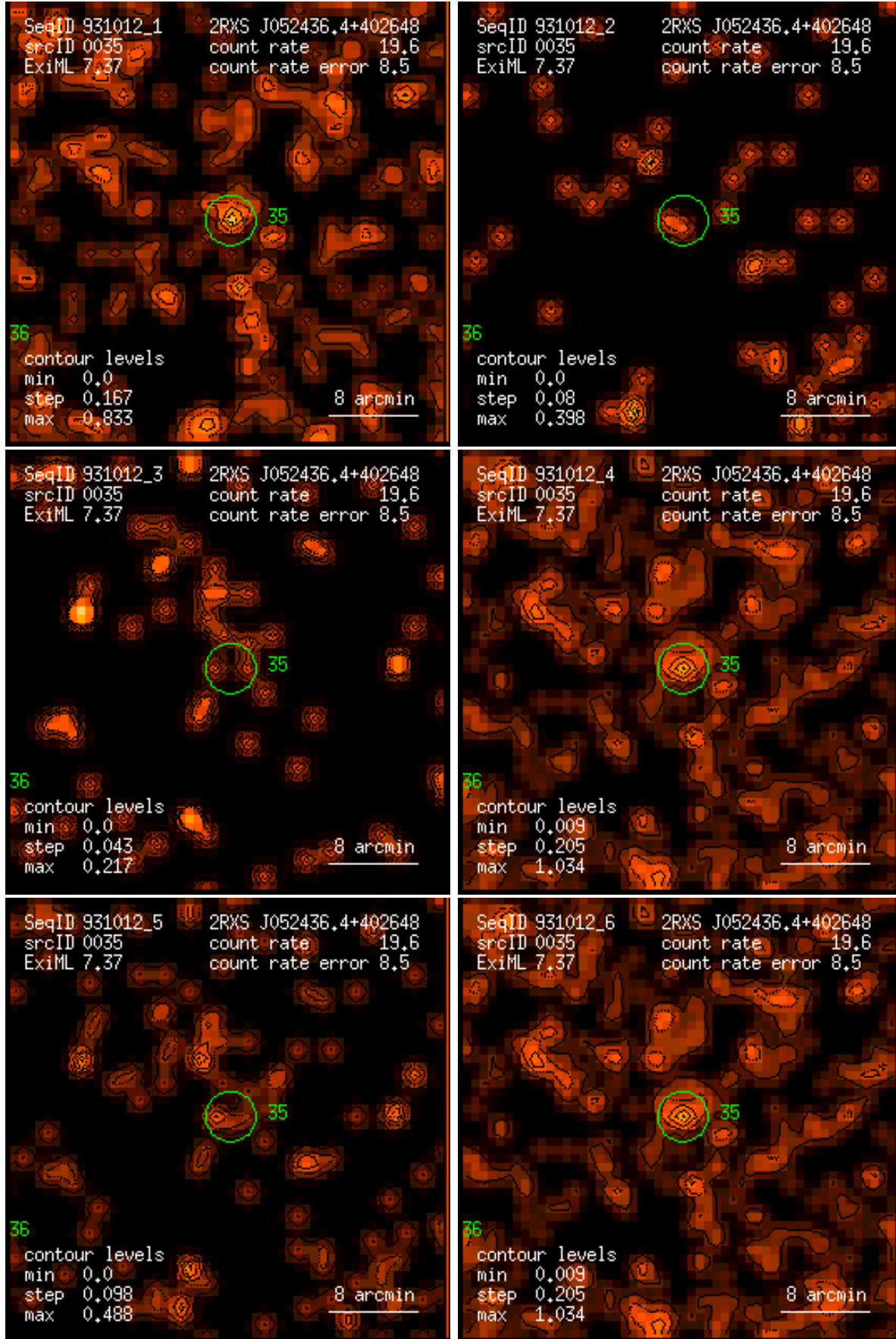
Figure 35: RASS 931012: detection 0035: band rate images, Gaussian filter: (1) PSPC channels 11 – 41, (2) 52 – 90, (3) 91 – 201, (4) 11 – 235, (5) 52 – 201, (6) 11 – 201. Broad band rates in counts/ks. Band rate contour levels in counts/ks/arcmin 2 .
